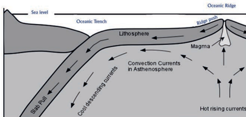
Figure 1.9: Convection currents in the Asthenosphere
