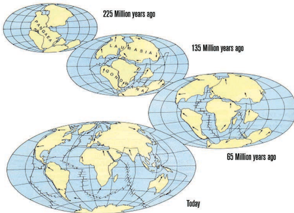
Figure 1.1: Continental Drift
