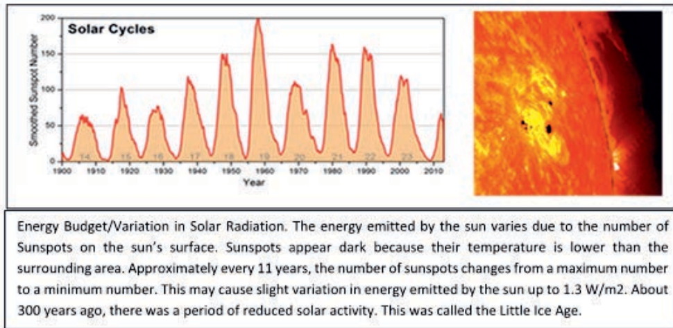
Figure 2.5: Solar cycle
