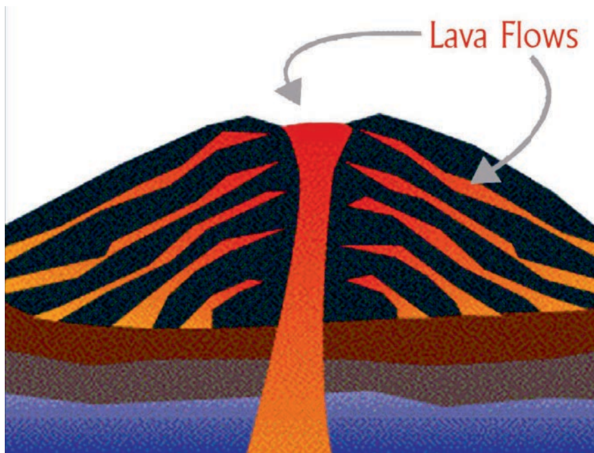
Figure 1.19: Shield volcano
