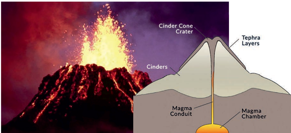
Figure 1.21: Cinder cone volcano
