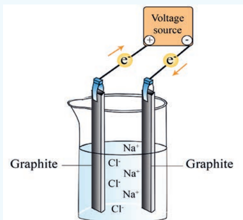
Figure 2. 3: Electrolytic cell containing molten sodium chloride.
