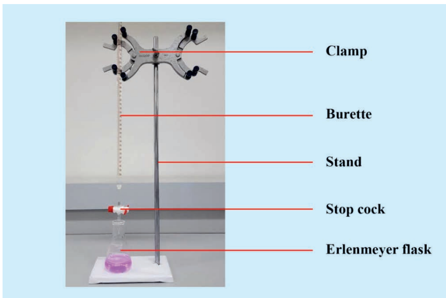
Figure 1.3: Titration Setup.
