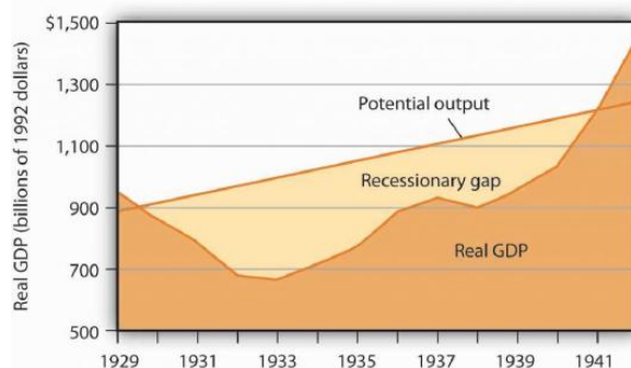
Figure 32.1 The Depression and the Recessionary Gap The dark-shaded area shows real GDP from 1929 to 1942, the upper line shows potential output, and the light-shaded area shows the difference between the two—the recessionary gap. The gap nearly closed in 1941; an inflationary gap had opened by 1942. The chart suggests that the recessionary gap remained very large throughout the 1930s.
