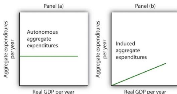
Figure 28.6 Autonomous and Induced Aggregate Expenditures Autonomous aggregate expenditures do not vary with the level of real GDP; induced aggregate expenditures do. Autonomous aggregate expenditures are shown by the horizontal line in Panel (a). Induced aggregate expenditures vary with real GDP, as in Panel (b).
