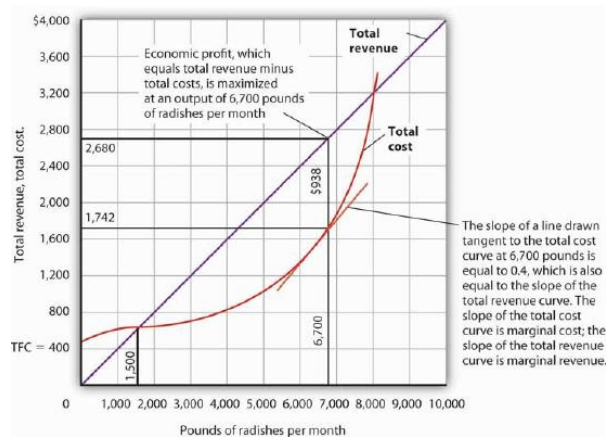
Figure 9.6 Total Revenue, Total Cost, and Economic Profit Economic profit is the vertical distance between the total revenue and total cost curves (revenue minus costs). Here, the maximum profit attainable by Tony Gortari for his radish production is $938 per month at an output of 6,700 pounds.
