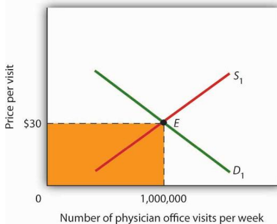
Figure 4.15 Total Spending for Physician Office Visits Total spending on physician office visits is $30 per visit multiplied by 1,000,000 visits per week, which equals $30,000,000. It is the shaded area bounded by price and quantity.
