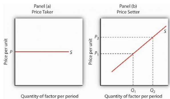
Figure 14.1 Factor Market Price Takers and Price Setters A price-taking firm faces the market-determined price P for the factor in Panel (a) and can purchase any quantity it wants at that price. A price-setting firm faces an upward-sloping supply curve S in Panel (b). The price-setting firm sets the price consistent with the quantity of the factor it wants to obtain. Here, the firm can obtain Q_1 units at a price P_1 , but it must pay a higher price per unit, P_2 , to obtain Q_2 units.
