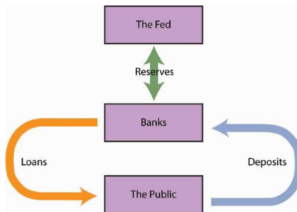
Figure 24.14 The Fed and the Flow of Money in the Economy Individuals and firms (the public) make deposits in banks; banks make loans to individuals and firms. The Fed can buy bonds to inject new reserves into the system, thus increasing bank lending, which creates new deposits, creating still more lending as the deposit multiplier goes to work. Alternatively, the Fed can sell bonds, withdrawing reserves from the system, thus reducing bank lending and reducing total deposits.
