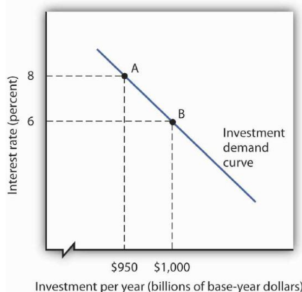
Figure 29.7 The Investment Demand Curve The investment demand curve shows the volume of investment spending per year at each interest rate, assuming all other determinants of investment are unchanged. The curve shows that as the interest rate falls, the level of investment per year rises. A reduction in the interest rate from 8% to 6%, for example, would increase investment from $950 billion to $1,000 billion per year, all other determinants of investment unchanged.
