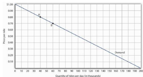
Figure 5.1 Responsiveness and Demand The demand curve shows how changes in price lead to changes in the quantity demanded. A movement from point A to point B shows that a $0.10 reduction in price increases the number of rides per day by 20,000. A movement from B to A is a $0.10 increase in price, which reduces quantity demanded by 20,000 rides per day.
