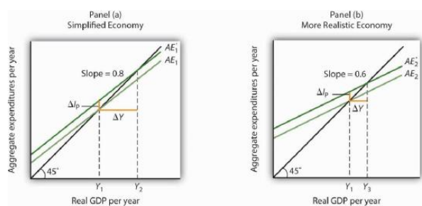
Figure 28.13 A Change in Autonomous Aggregate Expenditures: Comparison of a Simplified Economy and a More Realistic Economy In Panels (a) and (b), equilibrium real GDP is initially Y_1 . Then autonomous aggregate expenditures rise by the same amount, \Delta I_p . In Panel (a), the upward shift in the AE curve leads to a new level of equilibrium real GDP of Y_2 ; in Panel (b) equilibrium real GDP rises to Y_3 . Because equilibrium real GDP rises by more in Panel (a) than in Panel (b), the multiplier in the simplified economy is greater than in the more realistic one.
