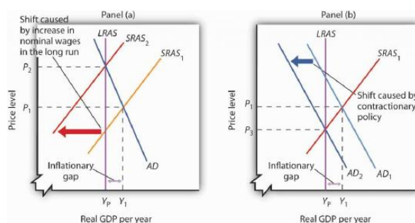
Figure 22.18 Alternatives in Closing an Inflationary Gap Panel (a) illustrates a gradual closing of an inflationary gap. Under a nonintervention policy, short-run aggregate supply shifts from SRAS_1 to SRAS_2 . Panel (b) shows the effects of contractionary policy to reduce aggregate demand from AD_1 to AD_2 in order to close the gap.
