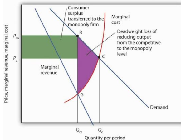
Figure 10.11 Perfect Competition, Monopoly, and Efficiency Given market demand and marginal revenue, we can compare the behavior of a monopoly to that of a perfectly competitive industry. The marginal cost curve may be thought of as the supply curve of a perfectly competitive industry. The perfectly competitive industry produces quantity Q_c and sells the output at price P_c . The monopolist restricts output to Q_m and raises the price to P_m .
