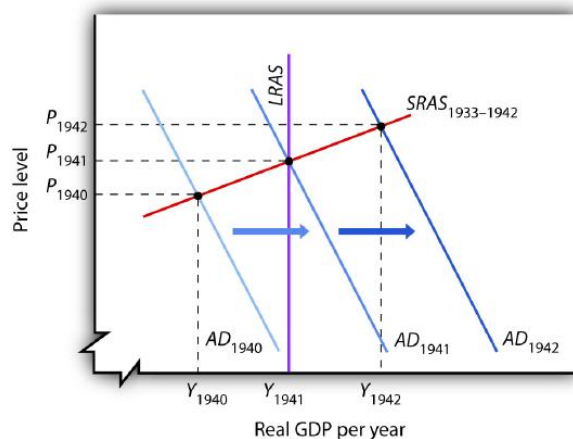
Figure 32.3 World War II Ends the Great Depression Increased U.S. government purchases, prompted by the beginning of World War II, ended the Great Depression. By 1942, increasing aggregate demand had pushed real GDP beyond potential output.
