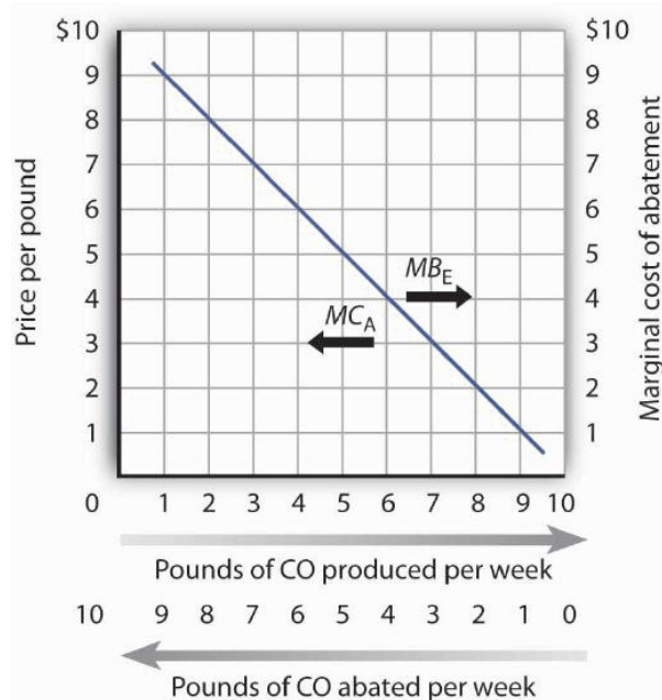
Figure 18.2 Abatement Costs and Demand A car emits an average of 10 pounds of CO per week when no restrictions are imposed—when the price of emissions is zero. The marginal cost of abatement ( MC_A ) is the cost of eliminating a unit of emissions; this is the interpretation of the curve when read from right to left. The same curve can be read from left to right as the marginal benefit of emissions ( MB_E ).
