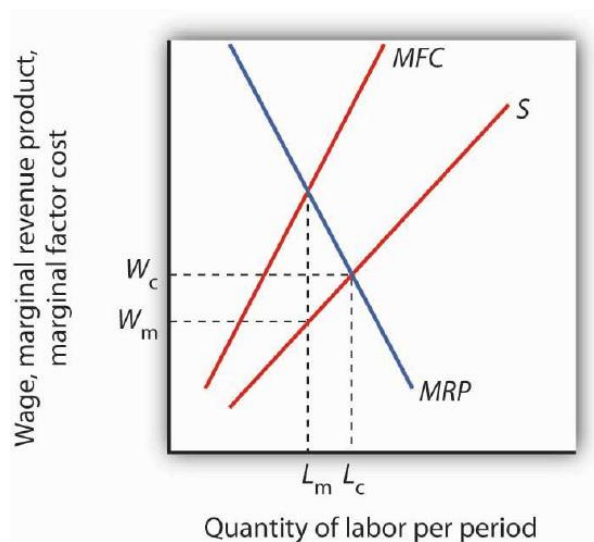
Figure 14.3 Monopsony Equilibrium Given the supply curve for labor, S , and the marginal factor cost curve, MFC , the monopsony firm will select the quantity of labor at which the MRP of labor equals its MFC . It thus uses L_m units of labor (determined by at the intersection of MRP and MFC ) and pays a wage of W_m per unit (the wage is taken from the supply curve at which L_m units of labor are available). The quantity of labor used by the monopsony firm is less than would be used in a competitive market ( L_c ); the wage paid, W_m , is lower than would be paid in a competitive labor market.
