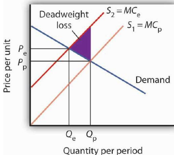
Figure 6.16 External Costs When firms in an industry generate external costs, the supply curve S_1 reflects only their private marginal costs, MC_p . Forcing firms to pay the external costs they impose shifts the supply curve to S_2 , which reflects the full marginal cost of the firms’ production, MC_e . Output is reduced and price goes up. The deadweight loss that occurs when firms are not faced with the full costs of their decisions is shown by the shaded area in the graph.
