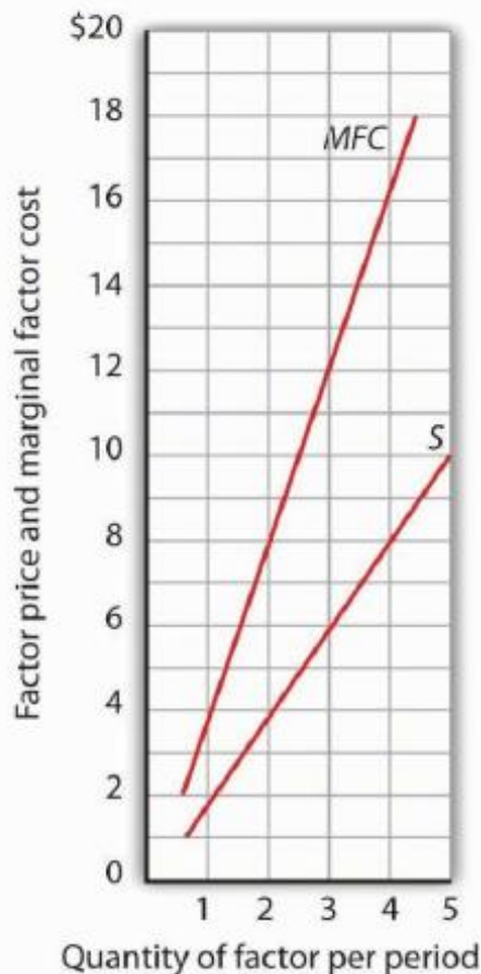
Figure 14.2 Supply and Marginal Factor Cost The table gives prices and quantities for the factor supply curve plotted in the graph. Notice that the marginal factor cost curve lies above the supply curve.
