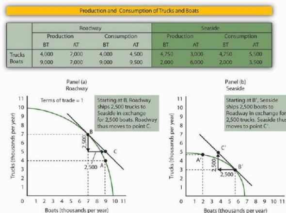
Figure 17.6 The Mutual Benefits of Trade Roadway and Seaside each consume more of both goods when there is trade between them. The table shows values of production before trade (BT) and after trade (AT). Here, the terms of trade are one truck in exchange for one boat. As shown in Panel (a) and in the exhibit's table, Roadway exports 2,500 trucks to Seaside in exchange for 2,500 boats and ends up consuming at point C, which is outside its production possibilities curve. Similarly, in Panel (b), Seaside ends up consuming at point C', which is outside its production possibilities curve. Trade allows both countries to consume more than they are capable of producing.
