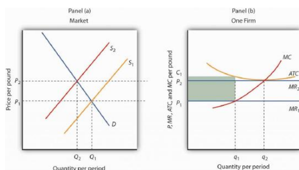
Figure 9.15 Eliminating Economic Losses in the Long Run Panel (b) shows that at the initial price P_1 , firms in the industry cannot cover average total cost ( MR_1 is below ATC ). That induces some firms to leave the industry, shifting the supply curve in Panel (a) to S_2 , reducing industry output to Q_2 and raising price to P_2 . At that price ( MR_2 ), firms earn zero economic profit, and exit from the industry ceases. Panel (b) shows that the firm increases output from q_1 to q_2 ; total output in the market falls in Panel (a) because there are fewer firms. Notice that in Panel (a) quantity is designated by uppercase Q , while in Panel (b) quantity is designated by lowercase q . This convention is used throughout the text to distinguish between the quantity supplied in the market ( Q ) and the quantity supplied by a typical firm ( q ).
