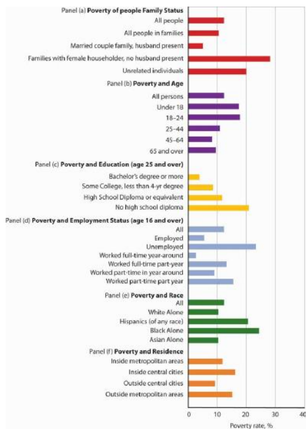
Figure 19.6 The Demographics of Poverty in the United States, 2006 Poverty rates in the United States vary significantly according to a variety of demographic factors. The data are for 2006.
