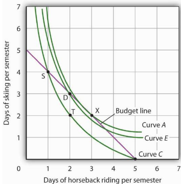
Figure 7.14 Applying the Marginal Decision Rule Suppose Ms. Bain is initially at point S. She is spending all of her budget, but she is not maximizing utility. Because her marginal rate of substitution exceeds the rate at which the market asks her to give up skiing for horseback riding, she can increase her satisfaction by moving to point D. Now she is on a higher indifference curve, E. She will continue exchanging skiing for horseback riding until she reaches point X, at which she is on curve A, the highest indifference curve possible.
