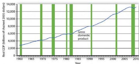
Figure 20.2 Expansions and Recessions, 1960–2010 The chart shows movements in real GDP since 1960. Recessions—periods of falling real GDP—are shown as shaded areas. On average, the annual rate of growth of real GDP over the period was 3.2% per year.
