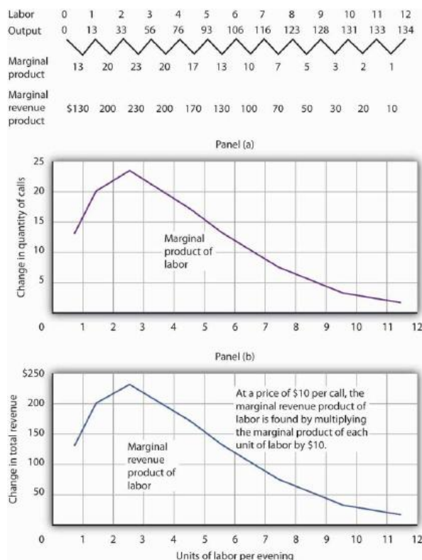
Figure 12.3 Marginal Product and Marginal Revenue Product The table gives the relationship between the number of accountants employed by TeleTax each evening and the total number of calls handled. From these values we derive the marginal product and marginal revenue product curves.
