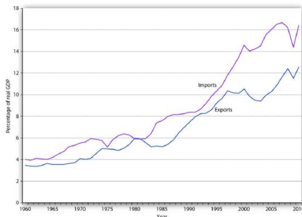
Figure 30.1 U.S. Exports and Imports Relative to U.S. Real GDP, 1960–2010 The chart shows exports and imports as a percentage of real GDP from 1960 through the third quarter of 2010.
