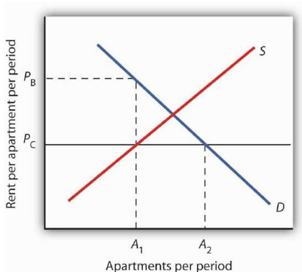
Figure 4.11 The Unintended Consequences of Rent Control Controlling apartment rents at P_C creates a shortage of (A_2 - A_1) apartments. For A_1 apartments, consumers are willing and able to pay P_B , which leads to various “backdoor” payments to apartment owners.
