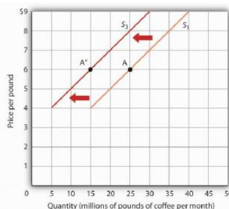
Figure 3.10 A Reduction in Supply A change in supply that reduces the quantity supplied at each price shifts the supply curve to the left. At a price of $6 per pound, for example, the original quantity supplied was 25 million pounds of coffee per month (point A). With a new supply curve S_3 , the quantity supplied at that price falls to 15 million pounds of coffee per month (point A').
