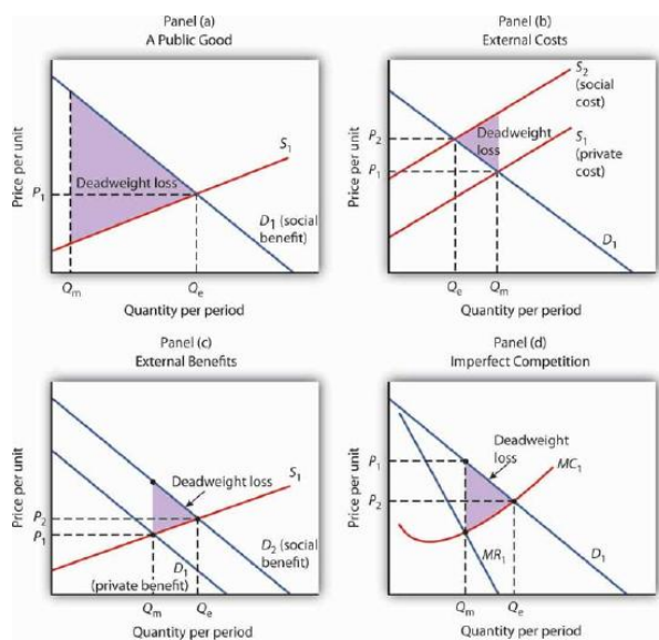
Figure 15.3 Correcting Market Failure In each panel, the potential gain from government intervention to correct market failure is shown by the deadweight loss avoided, as given by the shaded triangle. In Panel (a), we assume that a private market produces Q_m units of a public good. The efficient level, Q_e , is defined by the intersection of the demand curve D_1 for the public good and the supply curve S_1 . Panel (b) shows that if the production of a good generates an external cost, the supply curve S_1 reflects only the private cost of the good. The market will produce Q_m units of the good at price P_1 . If the public sector finds a way to confront producers with the social cost of their production, then the supply curve shifts to S_2 , and production falls to the efficient level Q_e . Notice that this intervention results in a higher price, P_2 , which confronts consumers with the real cost of producing the good. Panel (c) shows the case of a good that generates external benefits. Purchasers of the good base their choices on the private benefit, and the market demand curve is D_1 . The market quantity is Q_m . This is less than the efficient quantity, Q_e , which can be achieved if the activity that generates external benefits is subsidized. That would shift the market demand curve to D_2 , which intersects the market supply curve at the efficient quantity. Finally, Panel (d) shows the case of a monopoly firm that produces Q_m units and charges a price P_1 . The efficient level of output, Q_e , could be achieved by imposing a price ceiling at P_2 . As is the case in each of the other panels, the potential gain from such a policy is the elimination of the deadweight loss shown as the shaded area in the exhibit.
