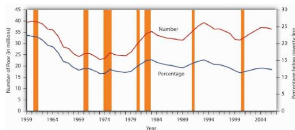
Figure 19.5 The Poverty Rate in the United States, 1959–2006 The curve shows the percentage of people who lived in households that fell below the poverty line in each year from 1959 to 2006. The poverty rate has generally fallen since 1959. Still, the poverty rate in the United States is greater than that of any other industrialized nation.
