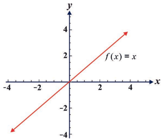
Figure 1.22 the graph of f( ) =
