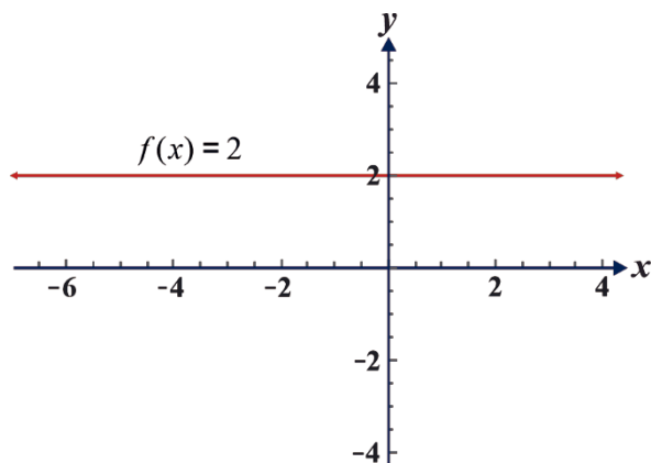
Figure 1.21 Graph of the constant function f( ) = 2
