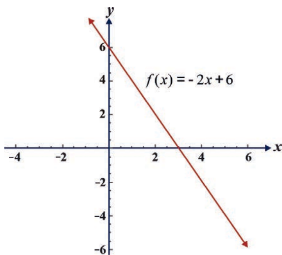
Figure 1.24 the graph of f(x) = -2x + 6
