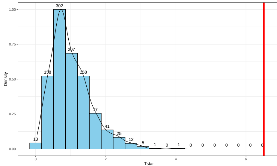
Figure 3.7: Histogram and density curve of the permutation distribution of the F -statistic with bold, vertical line for the observed value of the test statistic of 6.51.
