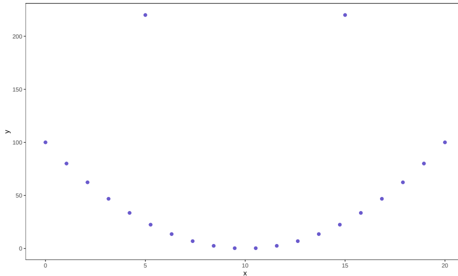
Figure 6.2: Scatterplot of an amusing (and strong) relationship that has r = 0 .
