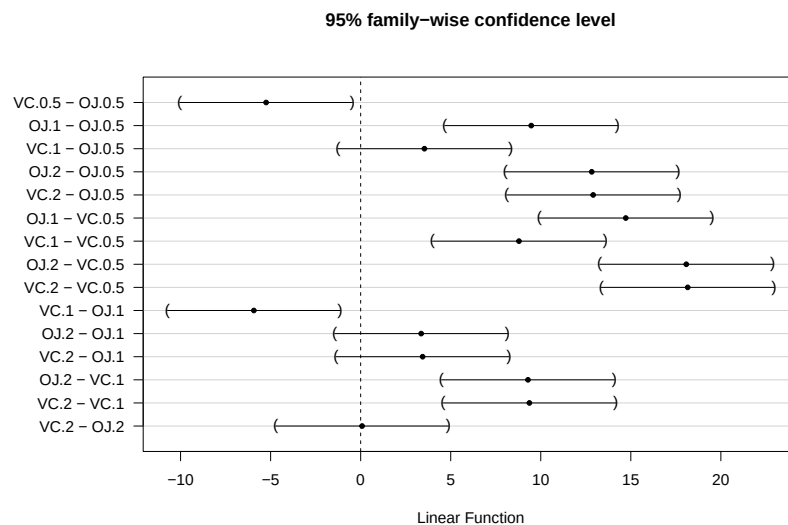
Figure 3.18: Graphical display of pair-wise comparisons from Tukey's HSD for the Guinea Pig data. Any confidence intervals that do not contain 0 provide strong evidence against the null hypothesis of no difference in the true means for that pair of groups.
