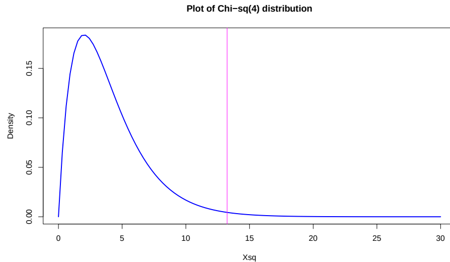
Figure 5.21: Plot of \chi^2 -distribution with 4 degrees of freedom.
