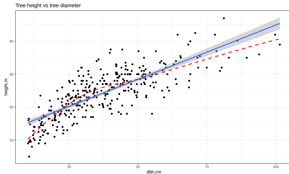
Figure 7.13: Scatterplot of tree height versus tree diameter.
