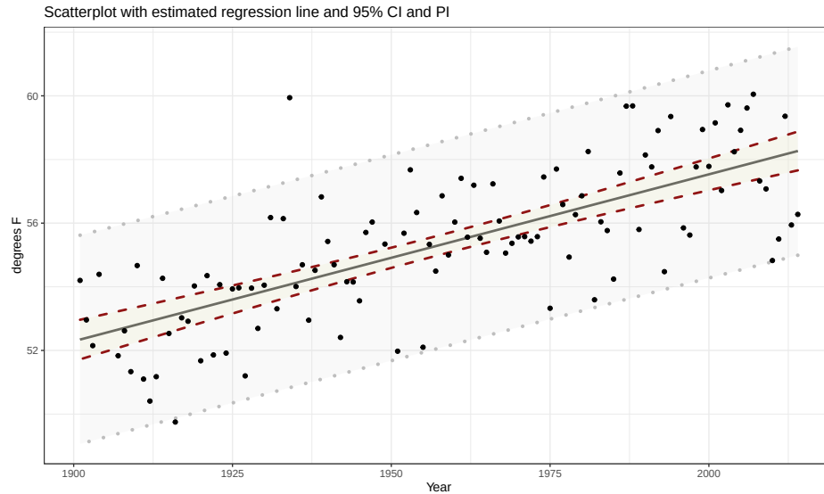
Figure 7.24: Estimated SLR for Bozeman temperature data with 95% confidence (dashed lines) and 95% prediction (lighter, dotted lines) intervals.
