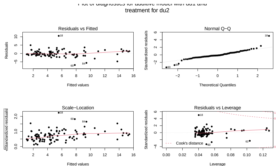
Figure 8.29: Diagnostic plots for the additive decibel tolerance model.
