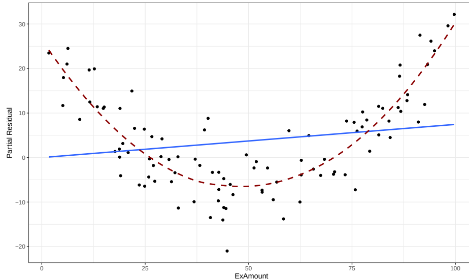
Figure 8.15: Plot of partial residual for ExAmount with the solid line for the MLR fit for this model component and the dashed line for the smoothing line that highlights the curvilinear relationship that the model failed to account for.
