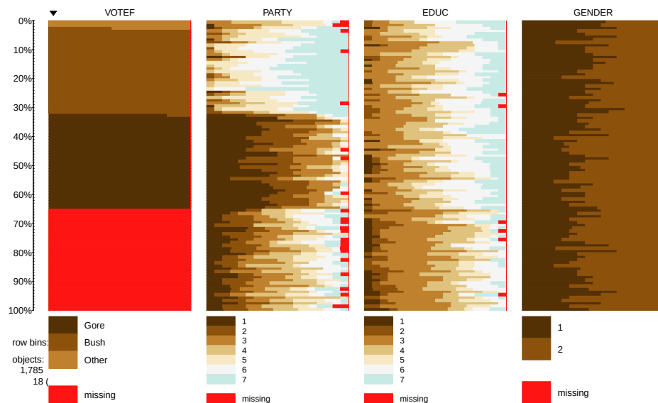
Figure 5.13: Tableplot of vote, party affiliation, education, and gender from election survey data. Note that missing observations are present in all variables except for Gender . Education is coded from 1 to 7 with higher values related to higher educational attainment. Gender code 1 is for male and 2 is for female.
