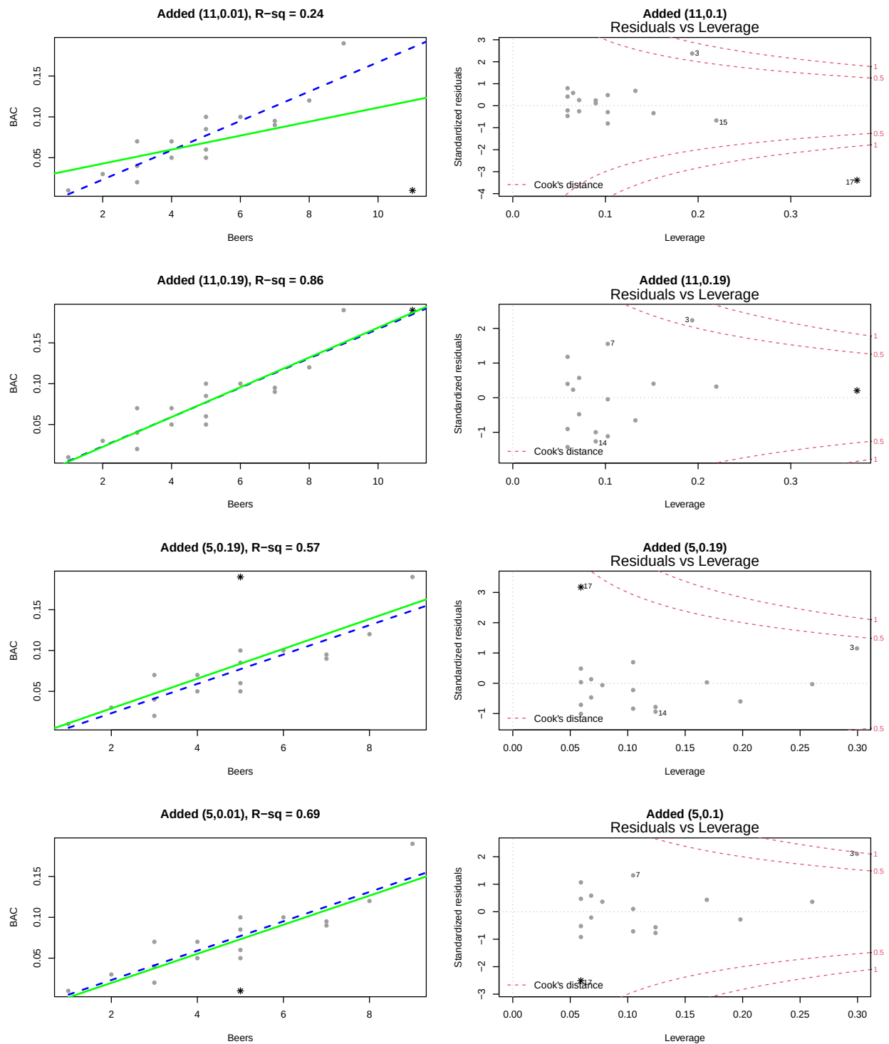
Figure 6.21: Plots exploring the impacts of moving a single additional observation in the BAC example. The added point is indicated with * and the original regression line is the dashed line in the left column.
