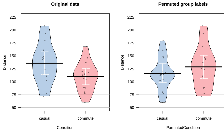
Figure 2.7: Pirate-plots of Distance responses versus actual treatment groups and permuted groups. Note how the responses are the same but that they are shuffled between the two groups differently in the permuted data set. With the smaller sample size, the 95% confidence intervals for each of the means are more clearly visible than with the original large data set.
