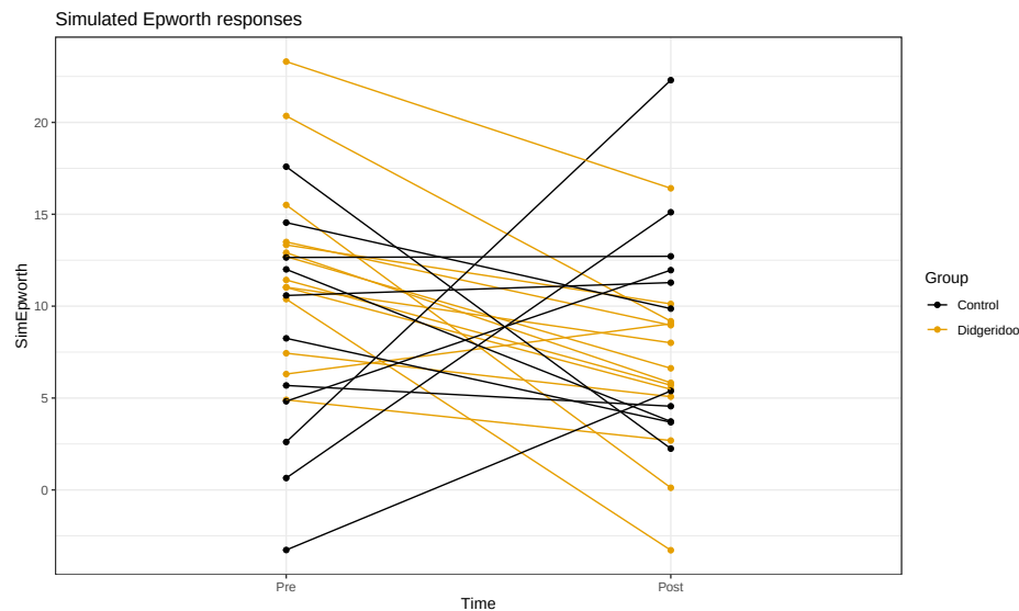
Figure 9.14: Plot of simulated data from the Two-Way ANOVA model that does not assume observations are on repeated measures on subjects to compare to the real data set. Even though the treatment levels seem to decrease on average, there is a much less clear relationship between the starting and ending values in the individuals.
