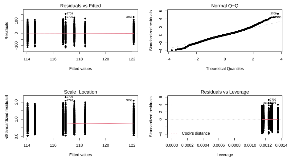
Figure 3.9: Default diagnostic plots for the full overtake data linear model.
