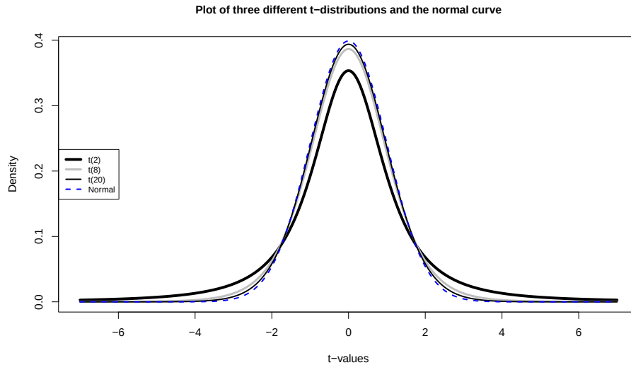
Figure 2.13: Plots of t -distributions with 2, 8, and 20 degrees of freedom and a normal distribution (dashed line). Note how the t -distributions get closer to the normal distribution as the degrees of freedom increase and at 20 degrees of freedom, the t -distribution almost matches a standard normal curve.
