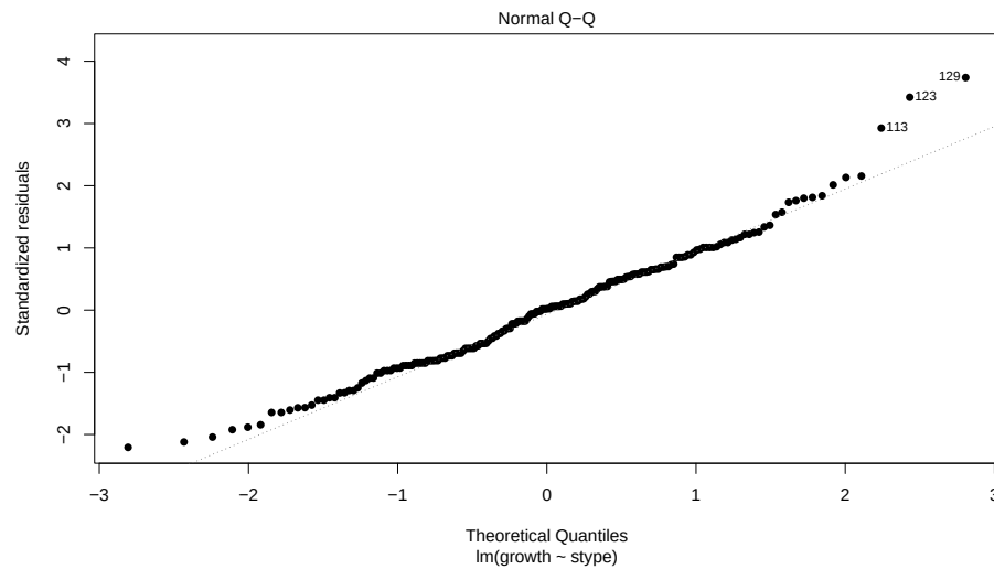
Figure 5.24: QQ-plot of standardized residuals from the One-Way ANOVA linear model.
