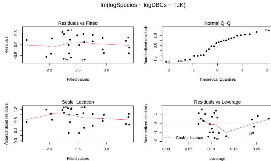
Figure 9.11: Diagnostic plots for the top AIC model.
