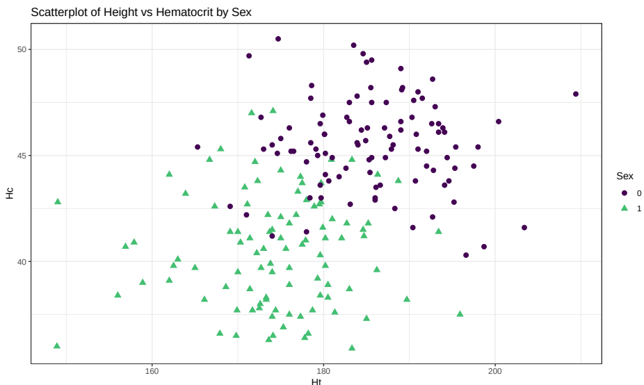
Figure 6.7: Scatterplot of athlete’s height and hematocrit by sex of athletes. Males were coded as 0s and females as 1s.
