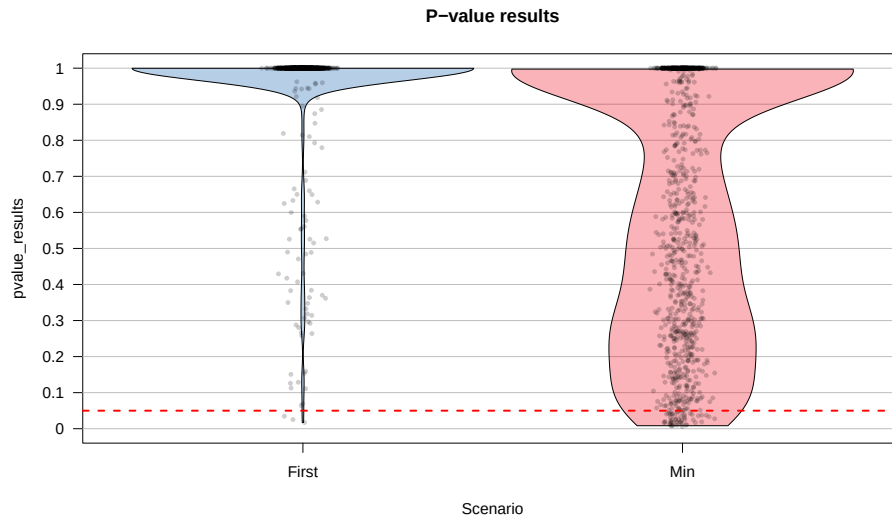
Figure 2.21: Pirate-plot of a simulation study results of p-values with Bonferroni correction.
