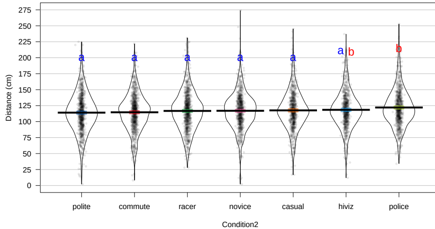
Figure 3.21: Pirate-plot of overtake distances by group, sorted by sample means with Tukey's HSD CLD displayed.
