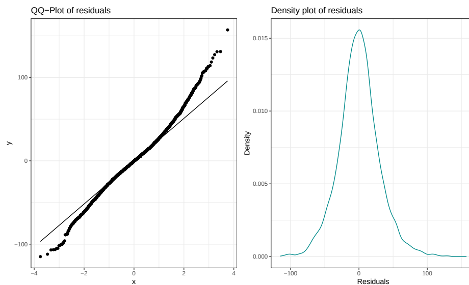
Figure 3.11: QQ-plot and density plot of residuals from the overtake data linear model.
