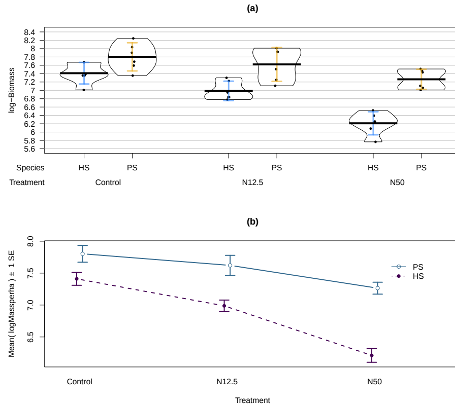
Figure 9.5: Pirate-plot and interaction plot of the log-Biomass responses by treatment and species.
