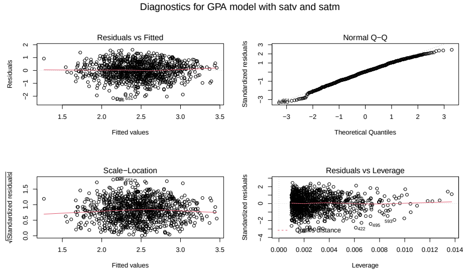
Figure 8.19: Diagnostic plots for the \text{fygpa} \sim \text{satm} + \text{satv} model.
