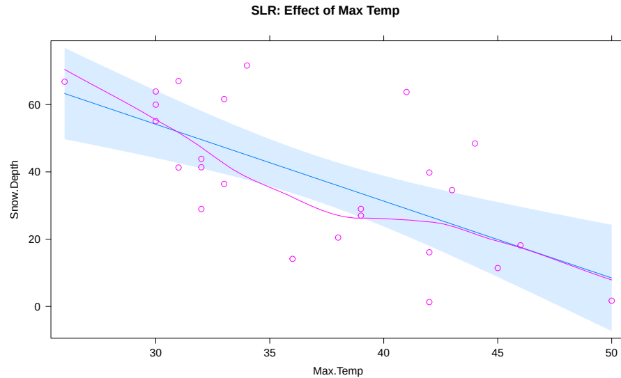
Figure 8.4: Plot of the estimated SLR model using Max Temp as predictor.
