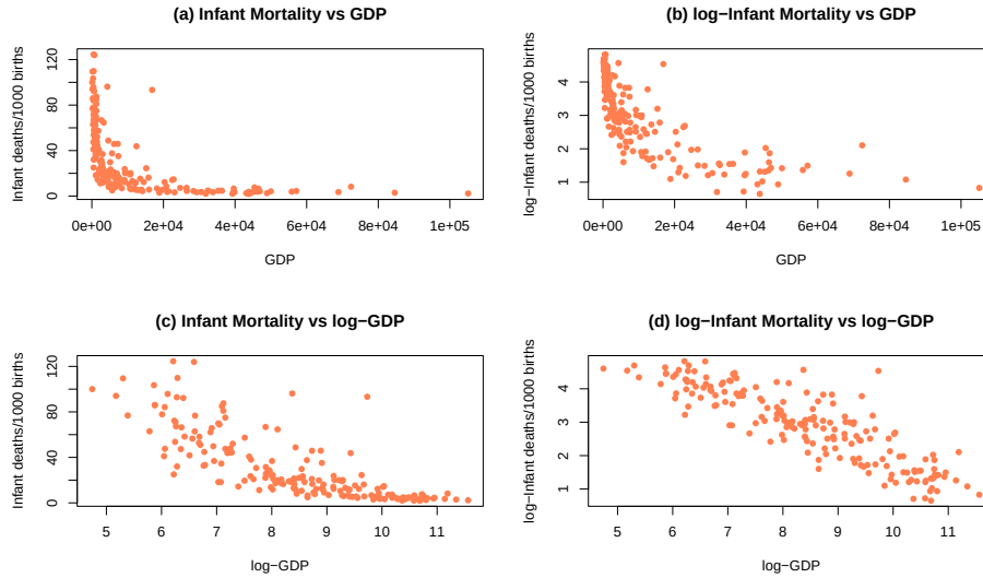
Figure 7.17: Scatterplots of Infant Mortality vs GDP under four different combinations of log-transformations.
