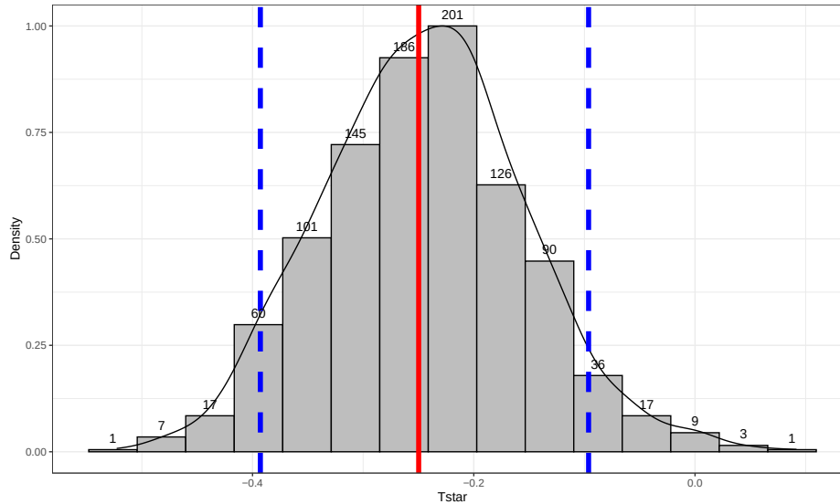
Figure 2.26: Histogram and density curve of bootstrap distribution of difference in sample mean GPAs (male minus female) with observed difference (solid vertical line) and quantiles that delineate the 90% confidence intervals (dashed vertical lines).
