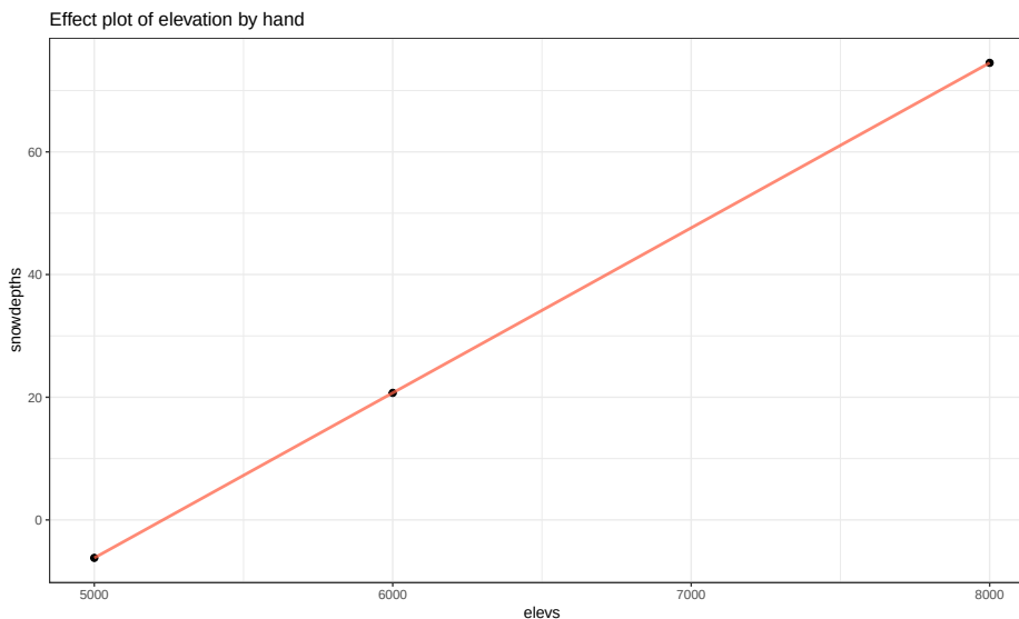
Figure 8.12: Term-plot for Elevation “by-hand”, holding temperature variables constant at their means.
