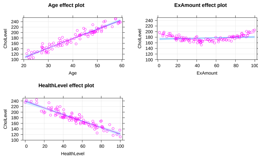
Figure 8.14: Term-plots with partial residuals for Cholesterol level versus three predictors (simulated data).
