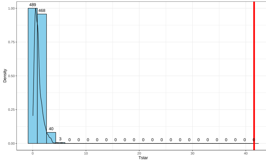
Figure 3.16: Histogram and density curve of permutation distribution for F -statistic for odontoblast growth data. Observed test statistic in bold, vertical line at 41.56.
