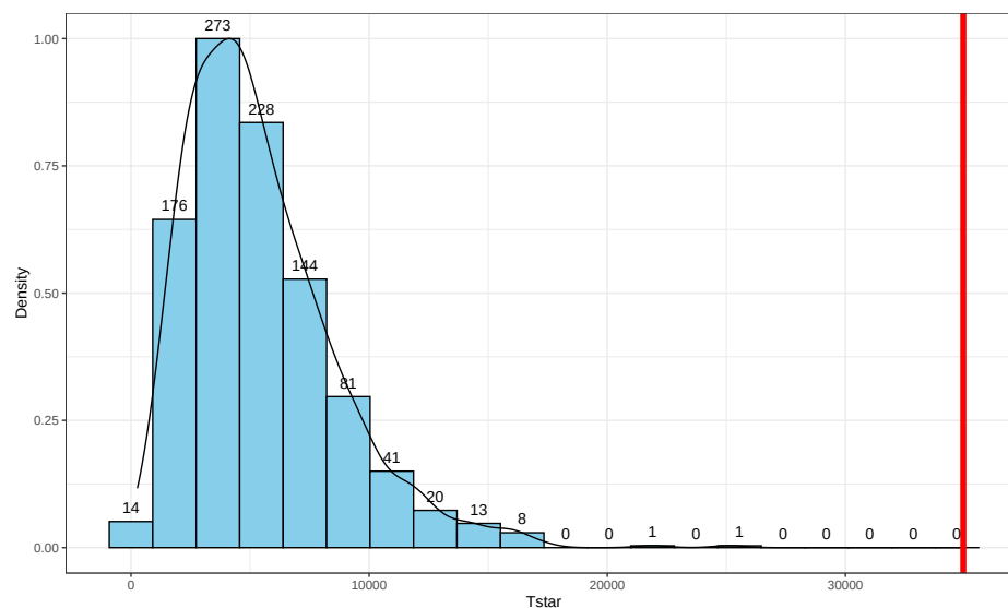
Figure 3.5: Histogram and density curve of permutation distribution of SS_A with the observed value of SS_A displayed as a bold, vertical line. The proportion of results that are as large or larger than the observed value of SS_A provides an estimate of the p-value.
