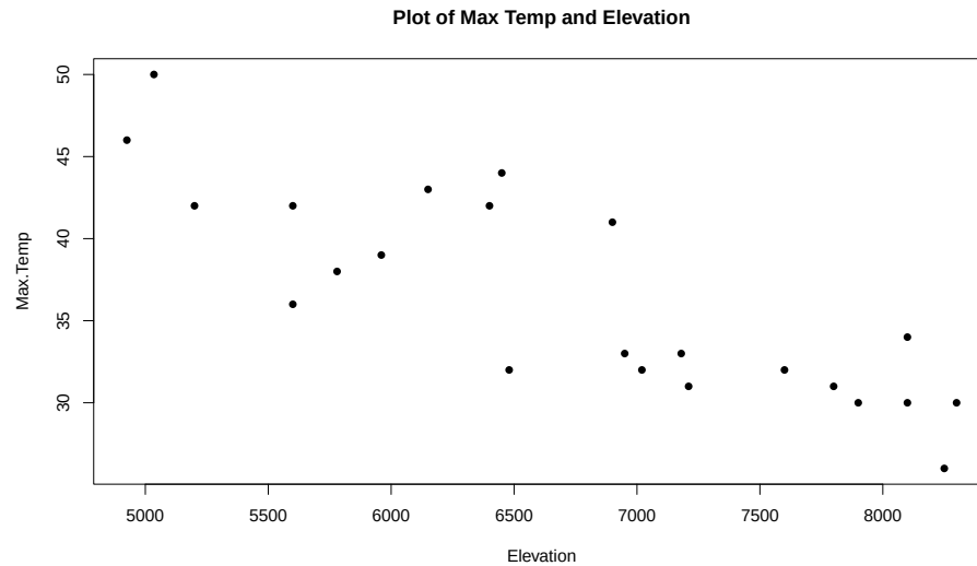
Figure 8.16: Scatterplot of observed Elevations and Maximum Temperatures for SNOTEL data.
