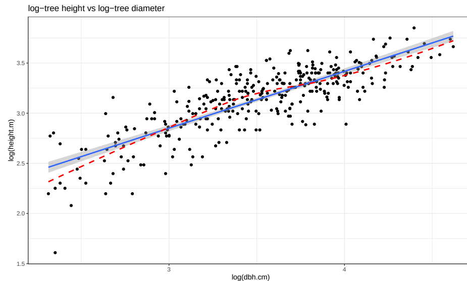
Figure 7.16: Scatterplot of \log(\text{tree height}) versus \log(\text{tree diameter}) .
