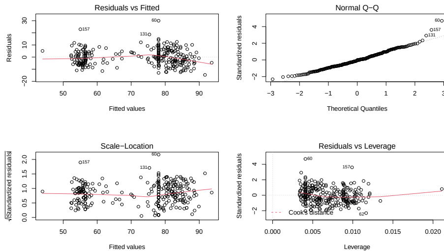
Figure 6.25: Diagnostic plots for Old Faithful waiting time model.
