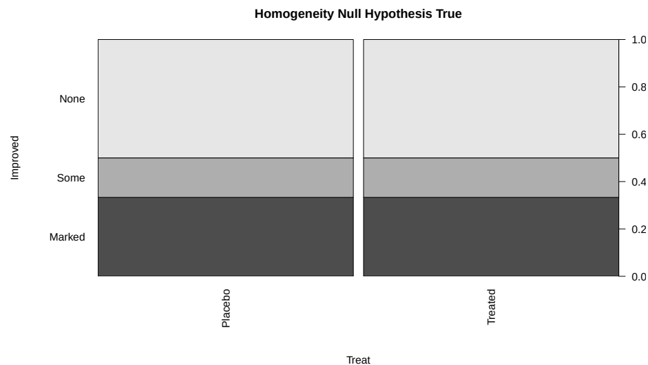
Figure 5.4: Plot of one way that the Arthritis proportions could have been if the null hypothesis had been true.
