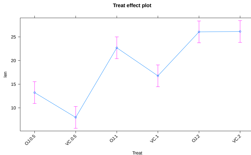
Figure 3.17: Effect plot of the One-Way ANOVA model for the odontoblast growth data, with rotated x-axis text for enhanced readability of the levels of the predictor variable.
