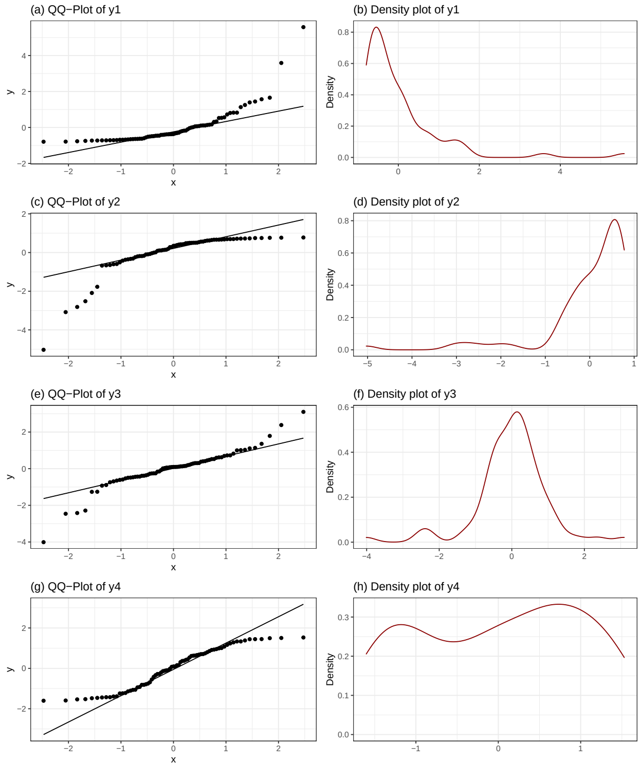
Figure 3.12: QQ-plots and density curves of four simulated distributions with different shapes.
