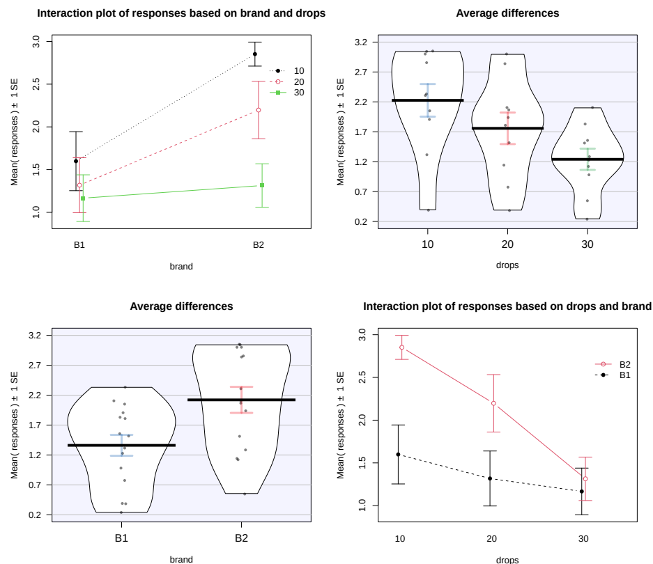
Figure 4.4: Interaction plot array of paper towel data with two different versions of interaction plots and pirate-plots of the responses versus each explanatory variable.
