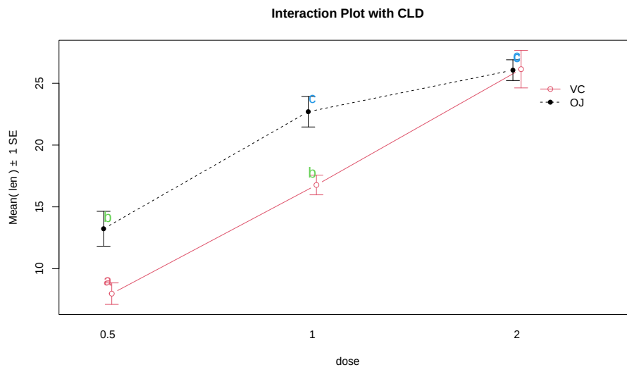
Figure 4.14: Interaction plot for Odontoblast data with added CLD from Tukey's HSD.
