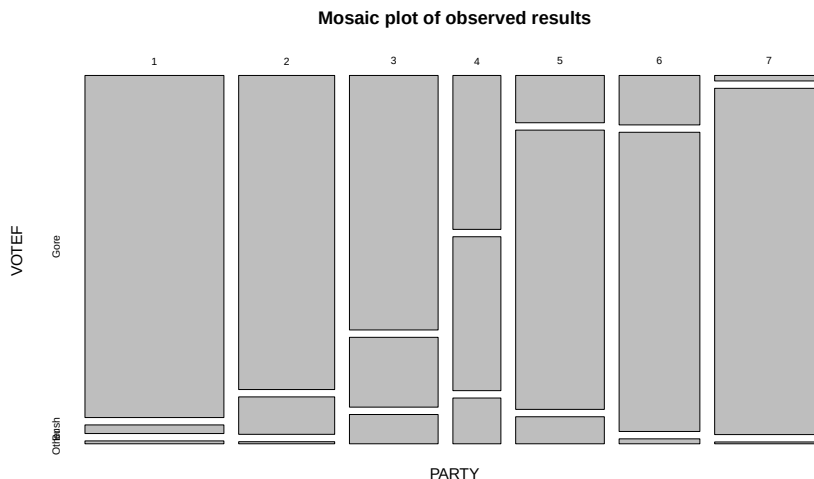
Figure 5.5: Mosaic plot of the 2000 election data comparing party affiliation and voting results.
