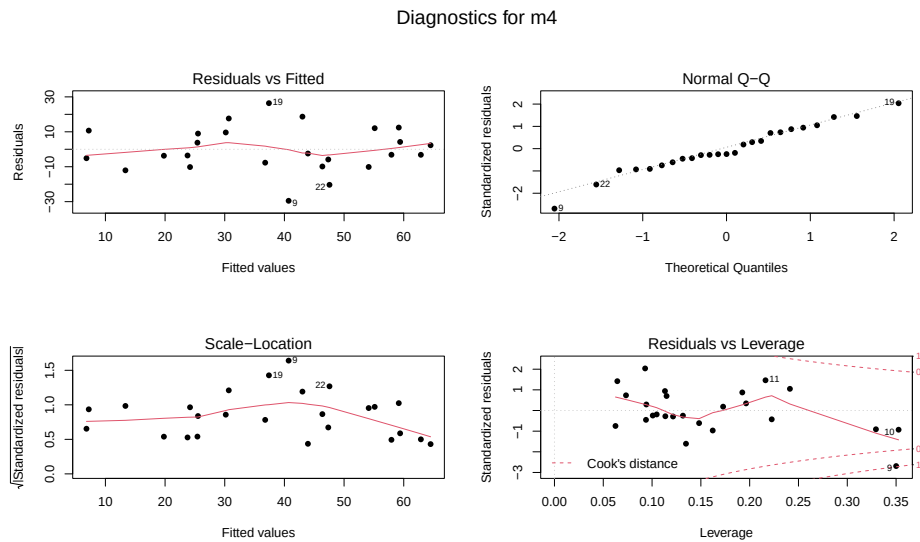
Figure 8.6: Diagnostic plots for model m4: \text{Snow.Depth} \sim \text{Elevation} + \text{Min.Temp} + \text{Max.Temp} .
