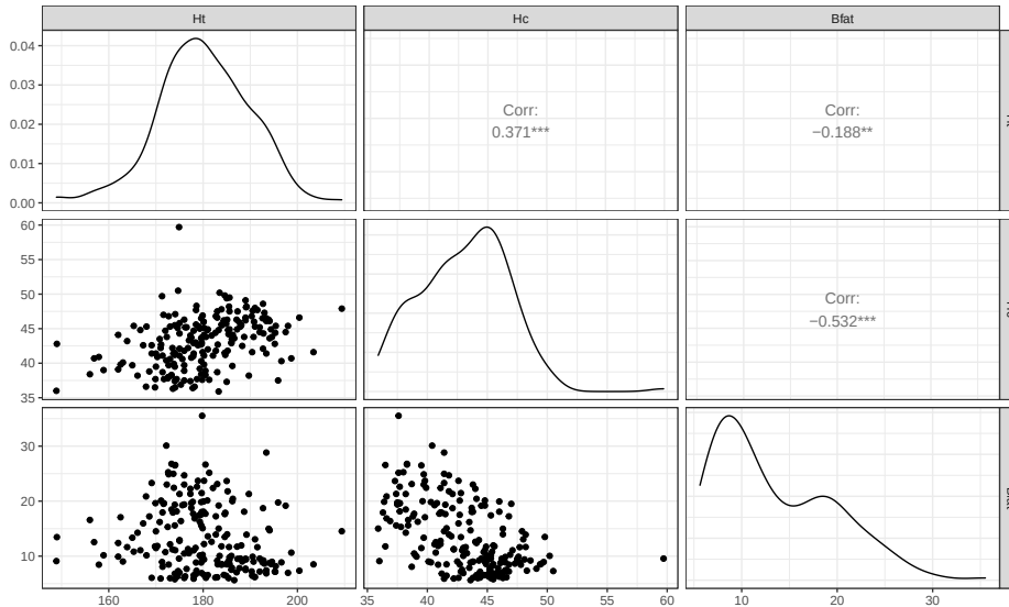
Figure 6.4: Scatterplot matrix of athlete data.
