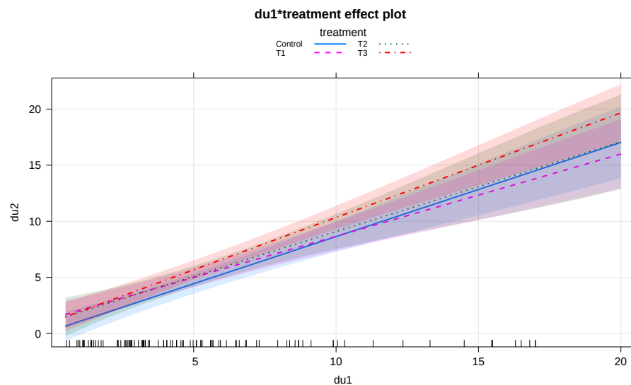
Figure 8.39: Term-plot for decibel tolerance interaction model (version 2). This plot is not printed in color because it is impossible to distinguish the four groups whether in color or black and white, although the lty = c(1:4) that provides four different line types does help a bit.
