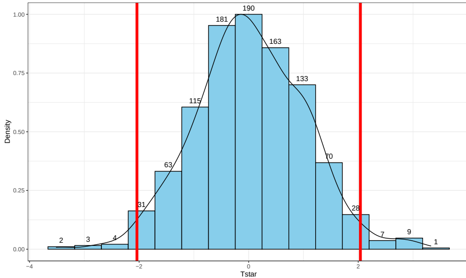
Figure 2.15: Permutation distribution of the t -statistic for n = 1,636 overtake data set.
