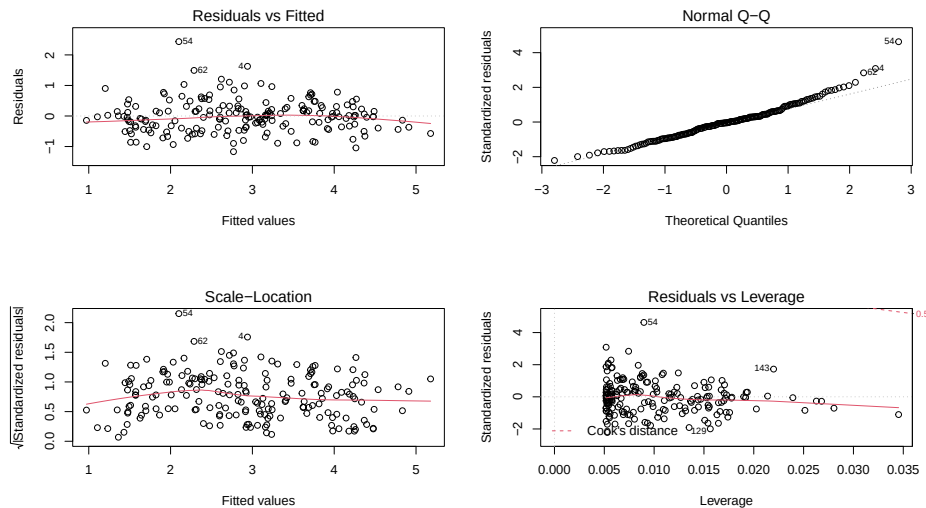
Figure 7.22: Diagnostic plots for the log-log infant mortality model.
