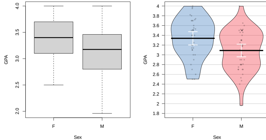
Figure 2.16: Side-by-side boxplot and pirate-plot of GPAs of Intermediate Statistics students by gender.
