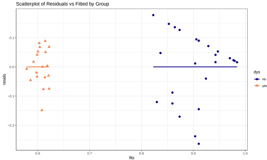
Figure 8.33: Plot of Residuals vs Fitted from interaction dyslexia data model with groups indicated.
