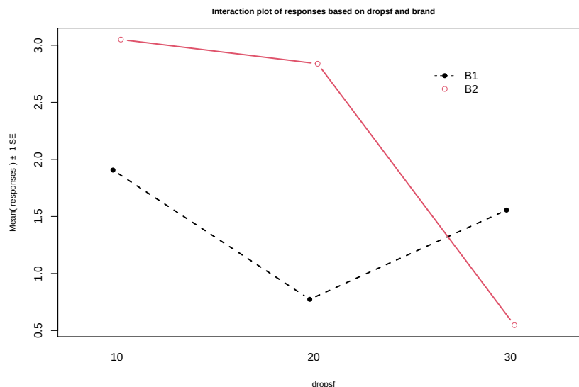
Figure 4.21: Interaction plot in paper towel data set with no replication.
