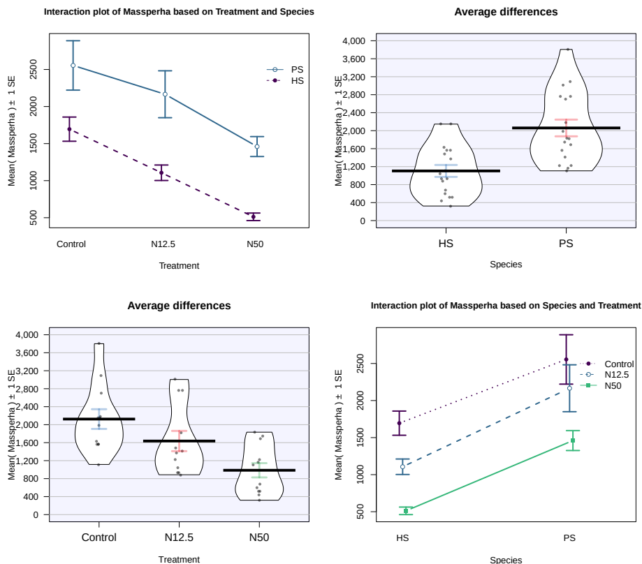
Figure 9.3: Interaction plot of biomass responses by treatment and species.
