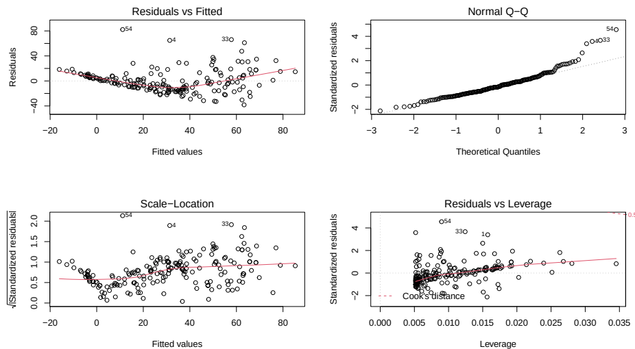
Figure 7.20: Diagnostics plots of the infant mortality model with \log(\text{GDP}) .
