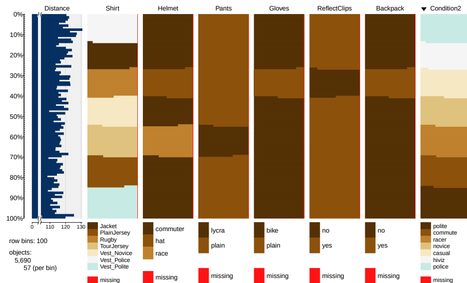
Figure 4.23: Tableplot of the full overtake data set sorted by outfit worn ( Condition2 ).
