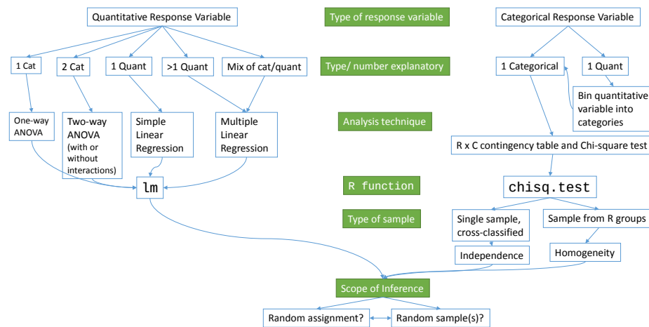
Figure 9.1: Schematic of methods covered.
