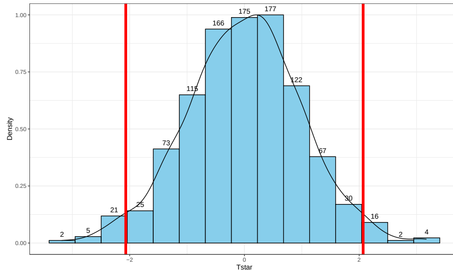
Figure 2.12: Permutation distribution of the t -statistic.
