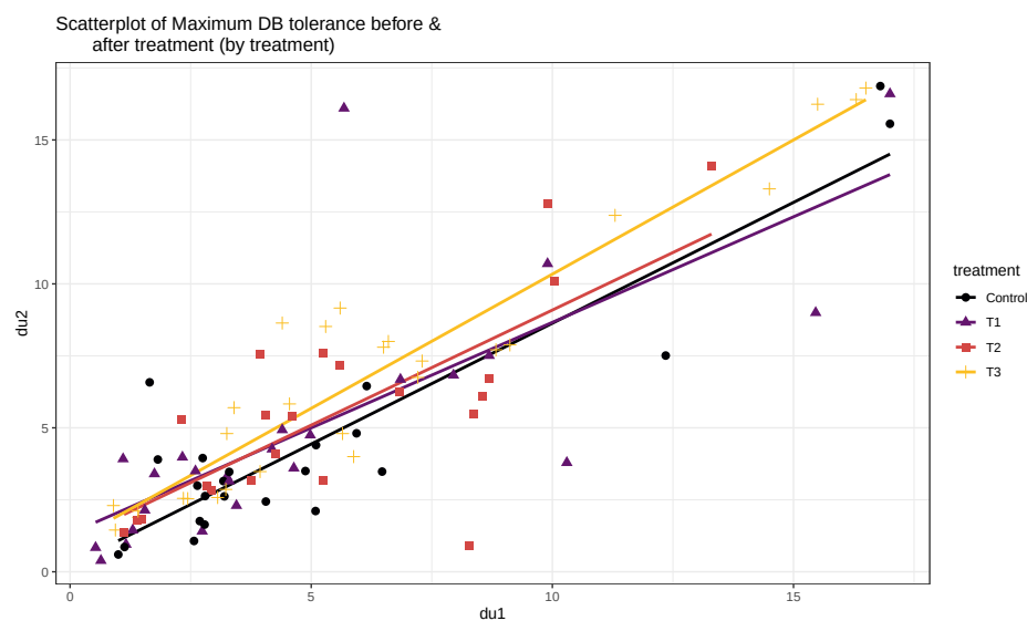
Figure 8.26: Scatterplot of post-treatment decibel tolerance ( du2 ) vs pre-treatment tolerance ( du1 ) by treatment level (4 groups).
