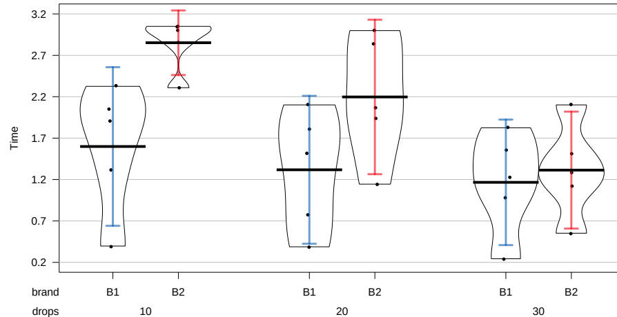
Figure 4.1: Pirate-plot of paper towel data by Brand (first row of x -axis) and Drops (second row of x -axis).
