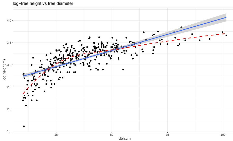
Figure 7.14: Scatterplot of \log(\text{tree height}) versus tree diameter.
