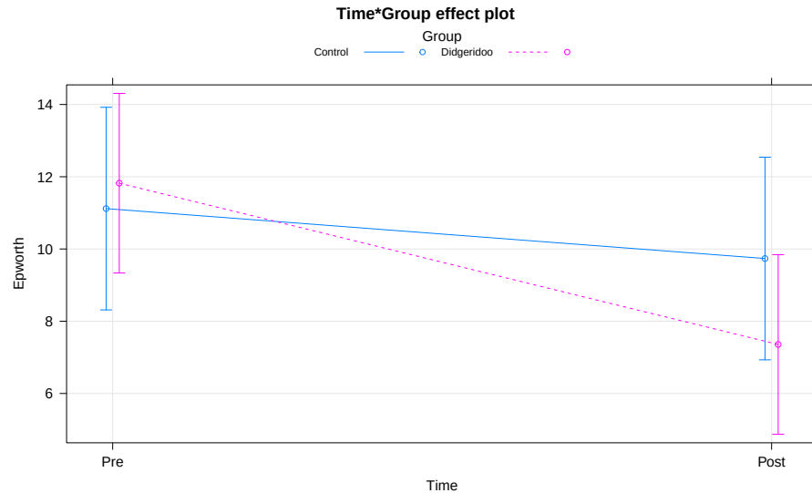
Figure 9.15: Term-plot of Time by Group interaction, results are from model that accounts for subject-to-subject variation in a mixed model.
