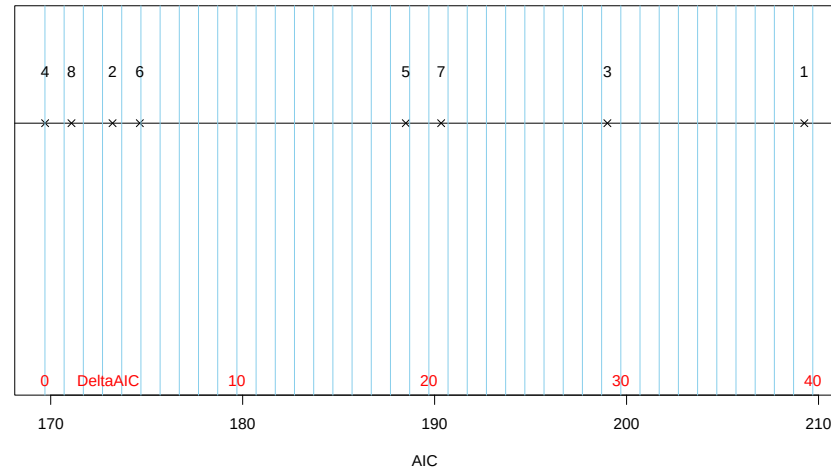
Figure 8.41: Display of AIC results on a number line with models indicated by their number in the dredge output. Note that the actual truth is unknown but further left in the plot corresponds to the models that are estimated to be closer to the truth and so there is stronger evidence for those models versus the others.
