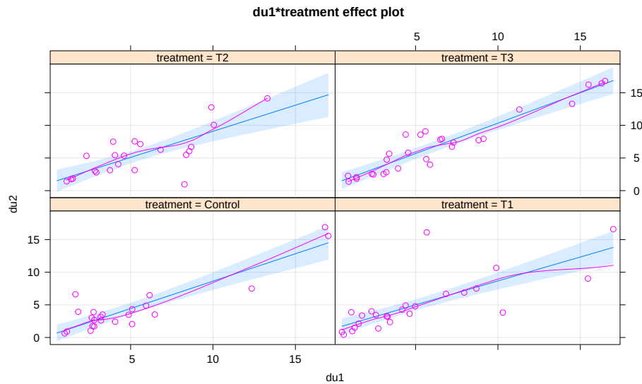
Figure 8.38: Term-plot for decibel tolerance interaction model with partial residuals (version 1).
