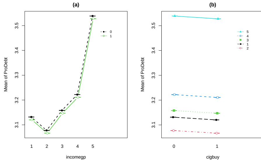
Figure 4.20: Illustration of the results from Table 4.3 showing the combined impacts of the components of the additive model for prodebt . Panel (a) uses income groups on the x-axis and different lines for cigarette buyers (1) or not (0). Panel (b) displays the different income groups as lines with the cigarette buying status on the x-axis.
