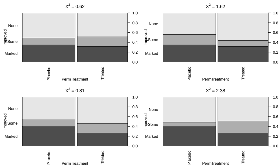
Figure 5.8: Stacked bar charts of four permuted Arthritis data sets that produced X^2 between 0.62 and 2.38.
