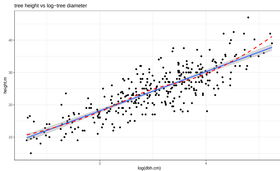
Figure 7.15: Scatterplot of tree height versus \log(\text{tree diameter}) .
