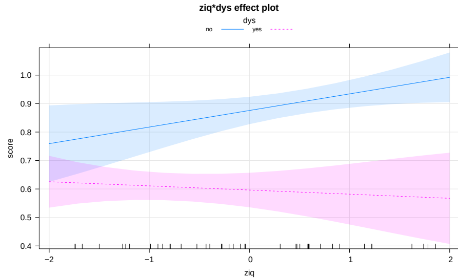
Figure 8.34: Term-plots for interaction model for reading scores using the multiline = T option to overlay the results for the two groups on one plot.
