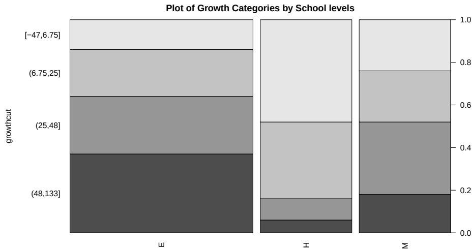
Figure 5.25: Stacked bar chart of the growth category responses by level of school.
