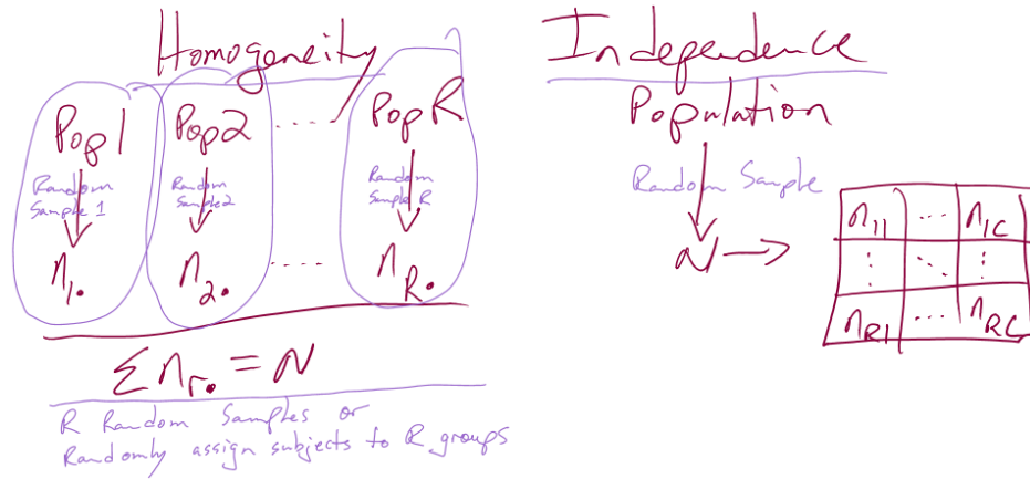
Figure 5.3: Diagram of the scenarios involved in Homogeneity and Independence tests. Homogeneity testing involves R random samples or subjects assigned to R groups. Independence testing involves a single random sample and measurements on two categorical variables.
