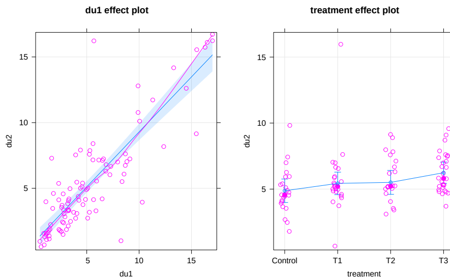
Figure 8.28: Term-plots of the additive decibel tolerance model with partial residuals.
