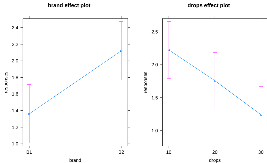
Figure 4.8: Term-plots of additive model for paper towel data. Left panel displays results for two brands and right panel for number of drops of water, each after controlling for the other.
