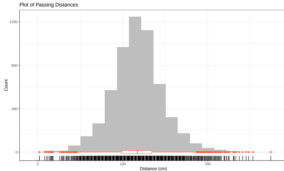
Figure 2.1: Histogram (with 20 bins), boxplot, and rug of passing distances (in cm).
