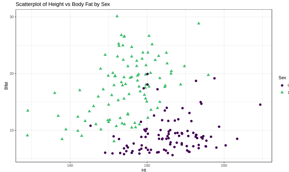
Figure 6.9: Scatterplot of athlete's body fat and height by sex.
