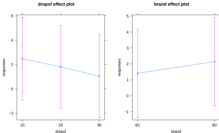
Figure 4.22: Term-plots for the additive model in paper towel data set with no replication.
