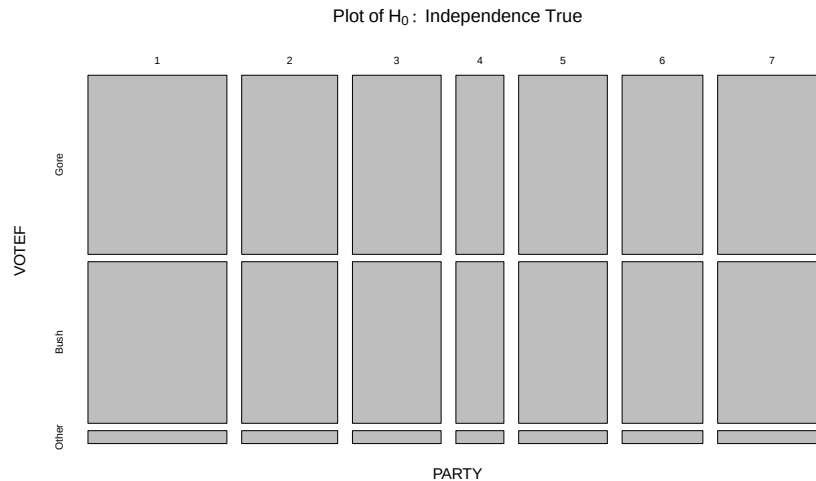
Figure 5.6: Mosaic plot of what the 2000 election data would look like if the null hypothesis of no relationship were true.
