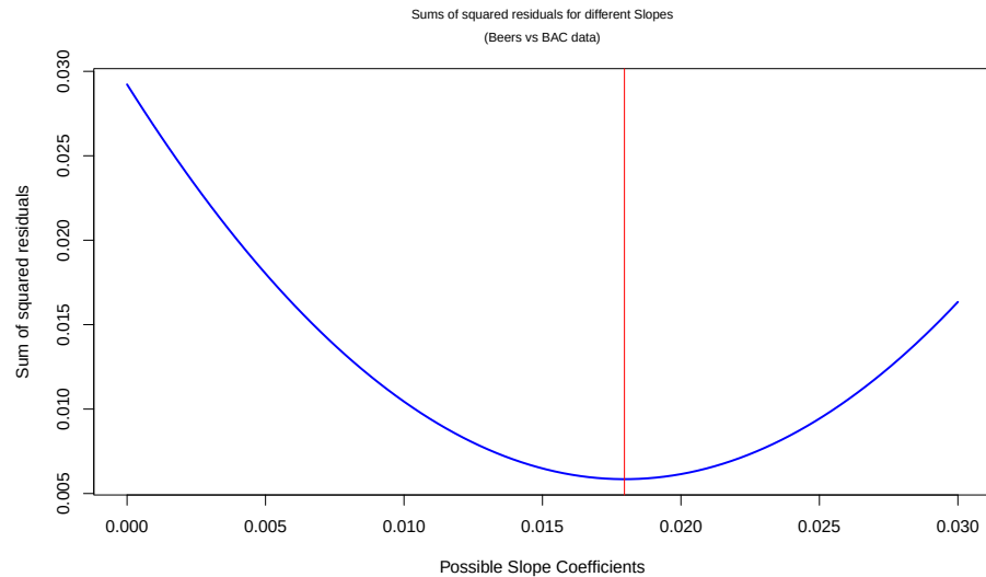
Figure 6.16: Plot of sum of squared residuals vs possible slope coefficients for Beers vs BAC data, with vertical line for the least squares estimate that minimizes the sum of squared residuals.
