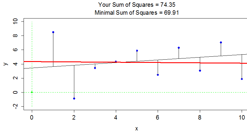
Figure 6.17: Results of running FindRegLine() where I didn't quite find the least squares line. The correct line is the bold (red) line and produced a smaller sum of squared residuals than the guessed thinner (black) line.
