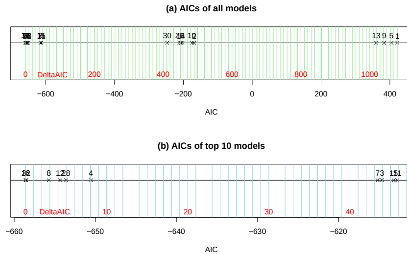
Figure 8.45: Display of AIC results on a number line with models indicated by their number in the dredge output. In more complex models, the dredge model numbers are just labels and not a meaningful numeration of the models being considered (there are 20 models considered here but labels go up to 32). Panel (a) presents results for all the models and panel (b) focuses just on the top 10 models so some differences in those models can be explored. Note that the spacing of the vertical grid lines in panel (a) are 10 AIC units and in (b) they are 1 AIC unit apart.
