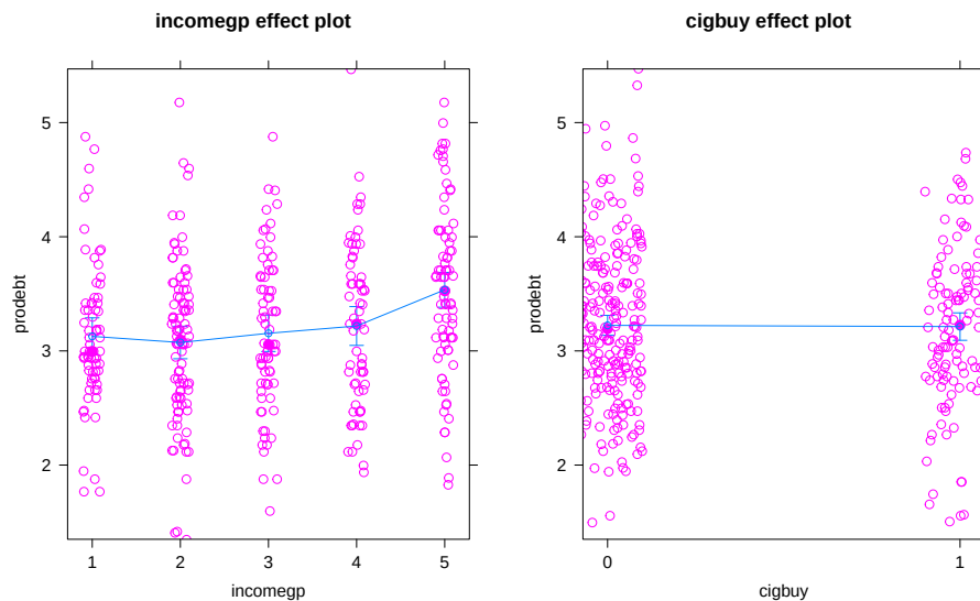
Figure 4.18: Term-plot for additive model for “prodebt” by income group and whether they buy cigarettes/not with partial residuals.
