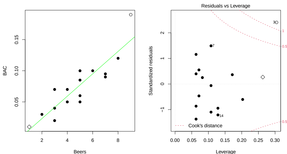
Figure 6.20: Scatterplot and Residuals vs Leverage plot for the real BAC data. Two high leverage points are flagged, with only one that has a Cook's D value over 1 ("o") and is indicated as influential.
