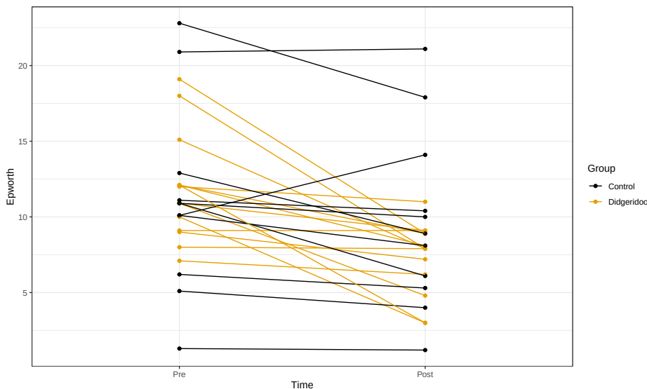
Figure 9.13: Plot of Epworth responses for each subject, initially and after four months, based on treatment groups with one line for each subject connecting observations made over time.
