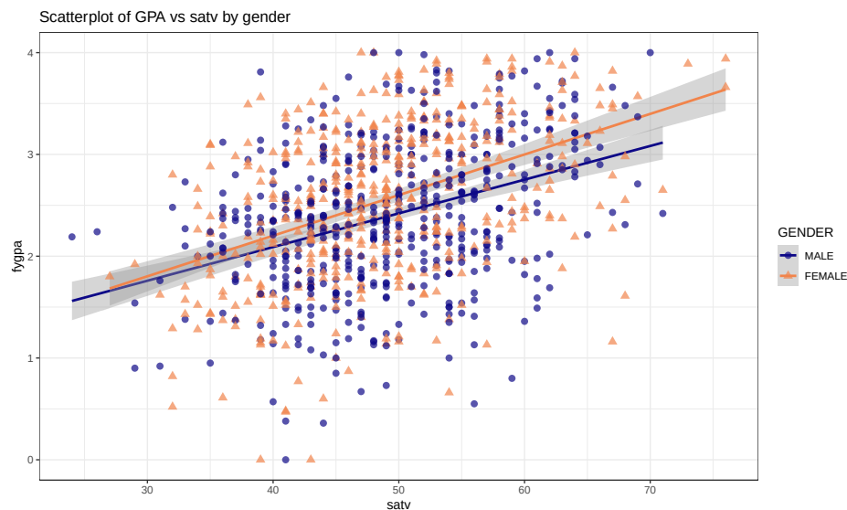
Figure 8.22: Plot of fygya vs satv by gender of students.
