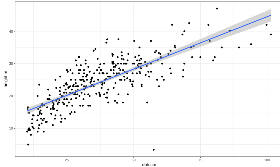
Figure 6.11: Scatterplot of tree heights (m) vs tree diameters (cm) with estimated straight line relationship (blue line) and 95% confidence interval (grey band).
