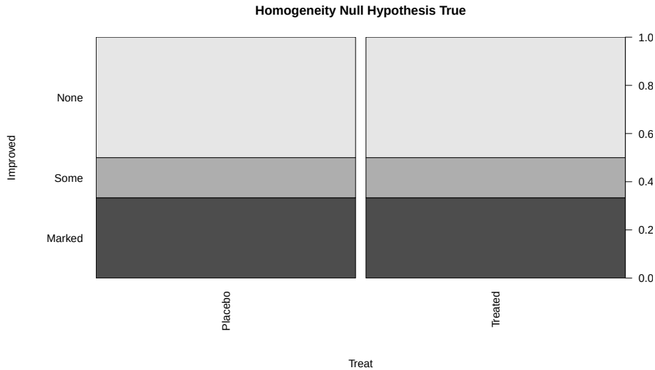
Figure 5.7: Stacked bar chart that could occur if the null hypothesis were true for the Arthritis study.
