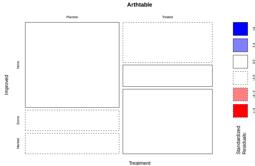
Figure 5.12: Mosaic plot of the Arthritis data with large standardized residuals indicated (actually, there were none that were indicated because all were less than 2). Note that dashed borders correspond to negative standardized residuals (observed less than expected) and solid borders are positive standardized residuals (observed more than expected).
