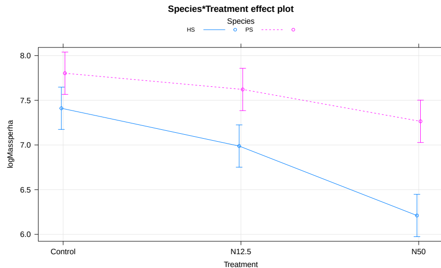
Figure 9.7: Term-plot of the interaction model for log-biomass.
