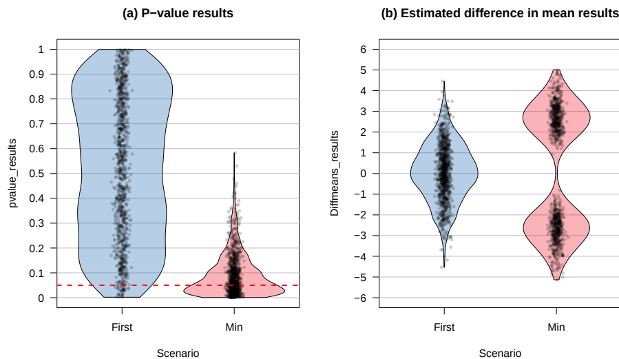
Figure 2.19: Pirate-plot of a simulation study results. Panel (a) contains the B = 1,000 p-values and (b) contains the B = 1,000 estimated differences in the means. Note that the estimated means and confidence intervals normally present in pirate-plots are suppressed here with inf.f.o = 0 , inf.b.o = 0 , avg.line.o = 0 because these plots are being used to summarize simulation results instead of an original data set.
