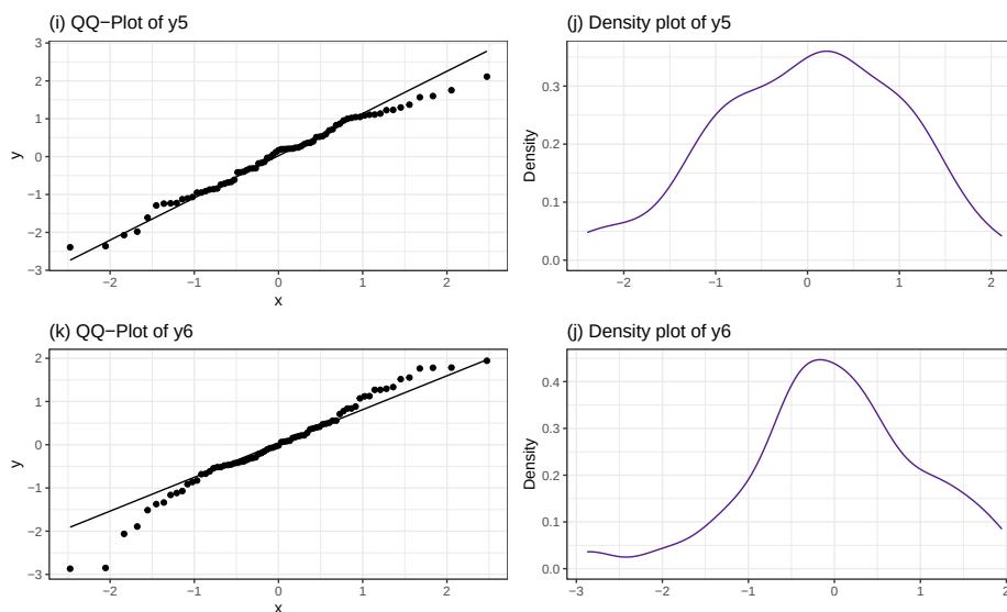
Figure 3.13: Two more simulated data sets, both generated from normal distributions.
