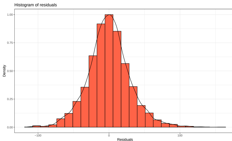
Figure 3.10: Histogram and density curve of the linear model raw residuals from the overtake data linear model.
