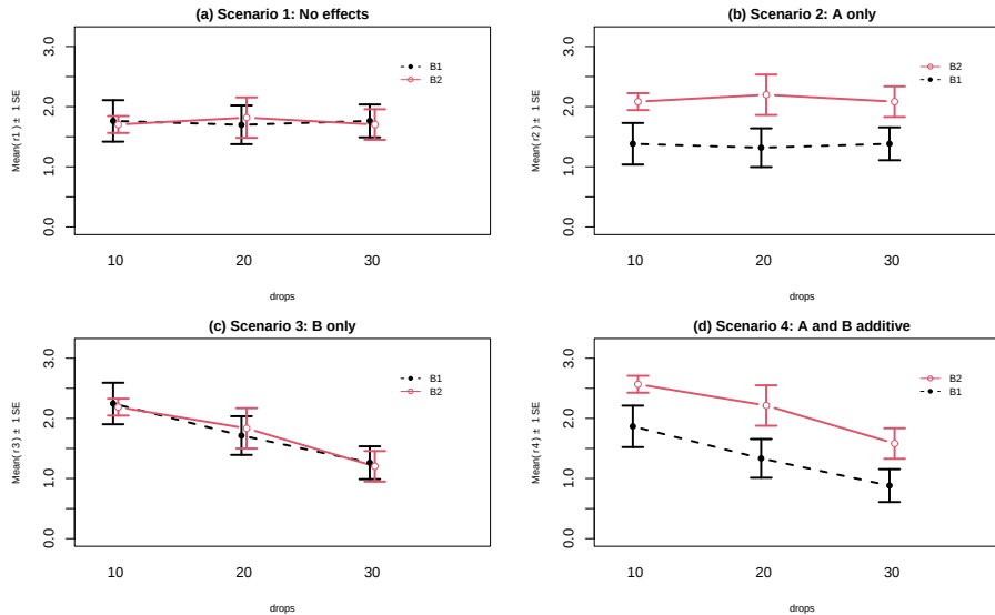
Figure 4.5: Interaction plots of four possible scenarios in the paper towel study.
