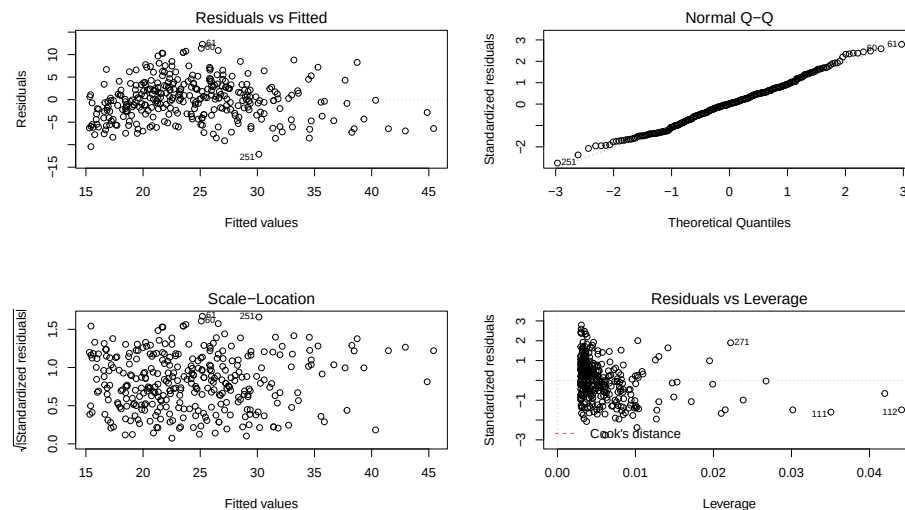
Figure 6.23: Diagnostics plots for tree height and diameter simple linear regression model.
