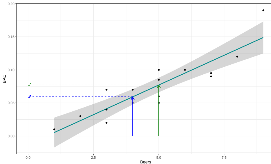
Figure 6.13: Scatterplot with estimated regression line (solid line) for the Beers and BAC data. The solid arrows indicate the predictor variable values of 4 and 5 beers and the dashed lines illustrate the predicted mean BAC for 4 and 5 beers consumed based on the SLR model.
