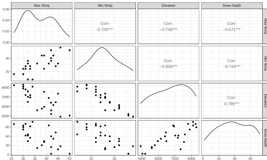
Figure 8.1: Scatterplot matrix of data from a sample of SNOTEL sites in April on four variables.
