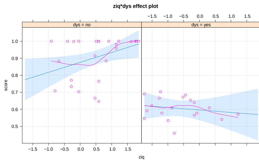
Figure 8.35: Term-plots for interaction model for reading scores with partial residuals and the results for the two groups in different panels of the plot.
