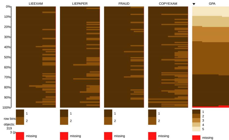
Figure 5.18: Tableplot of initial cheating and lying data set. Note that a few GPAs were missing in the data set.
