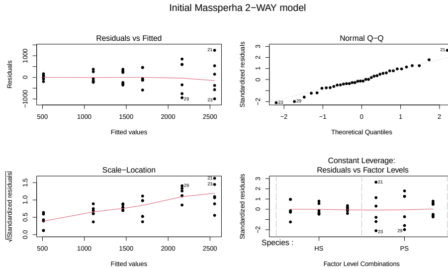
Figure 9.4: Diagnostic plots of treatment by species interaction model for Biomass.
