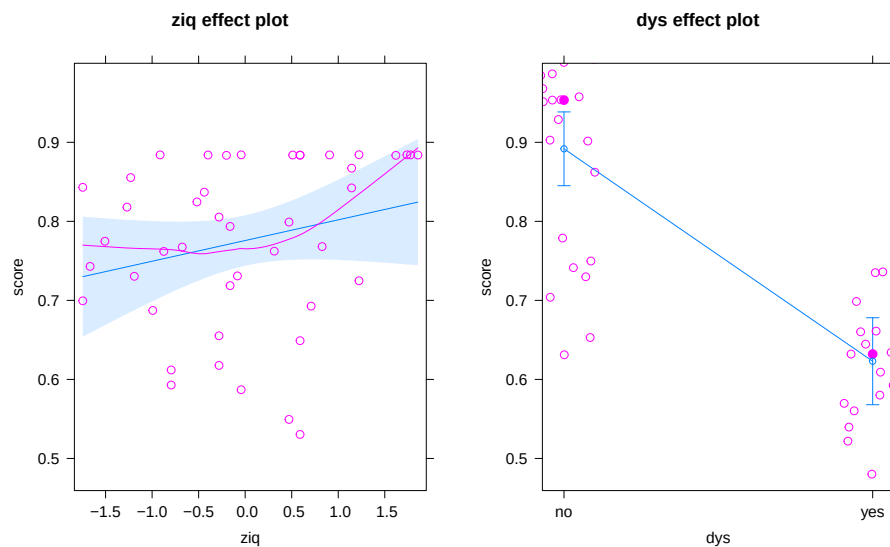
Figure 8.36: Term-plots for additive model for reading scores.
