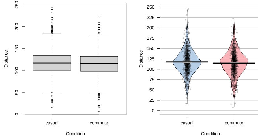
Figure 2.5: Boxplot and pirate-plot of the Distance responses on the reduced ddsub data set.
