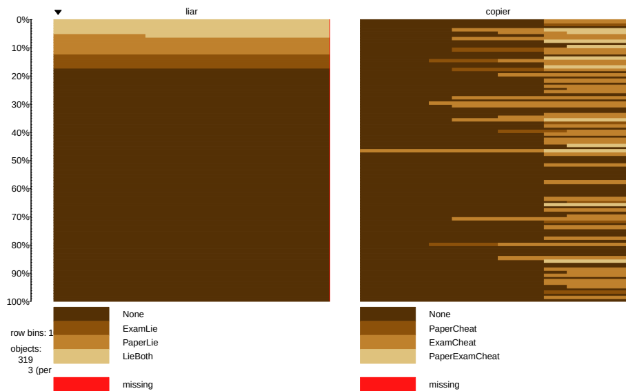
Figure 5.19: Tableplot of new variables liar and copier that allow exploration of relationships between different types of lying and cheating behaviors.
