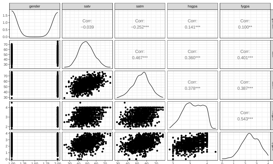
Figure 8.18: Scatterplot matrix of SAT and GPA data set.
