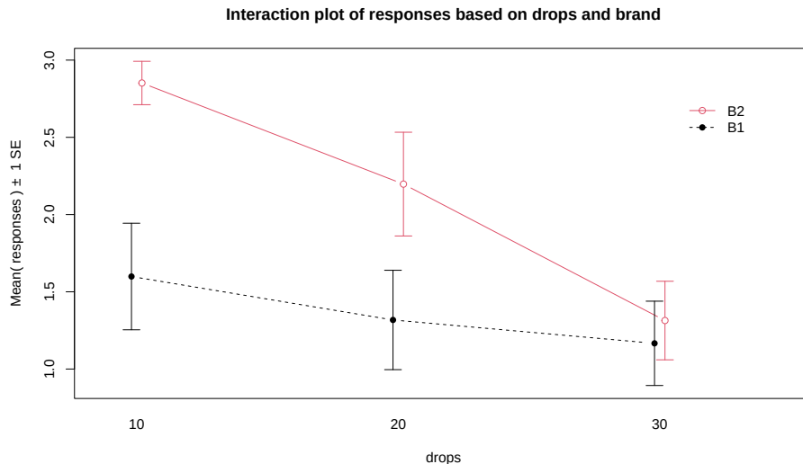
Figure 4.2: Interaction plot of the paper towel data with Drops on the x-axis and different lines based on Brand .
