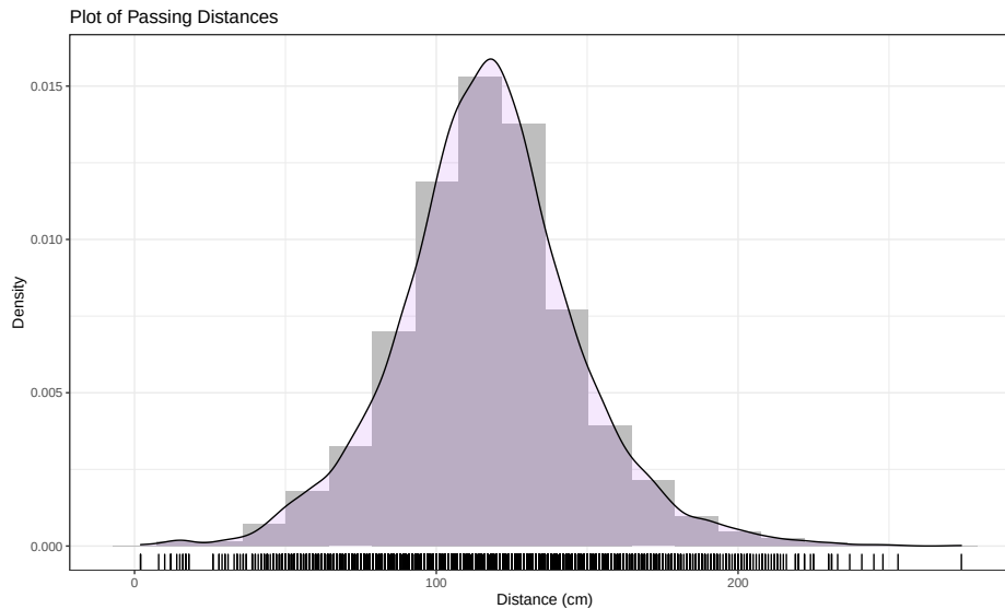
Figure 2.2: Histogram (density scaled), density curve, and rug plot of Distance responses.
