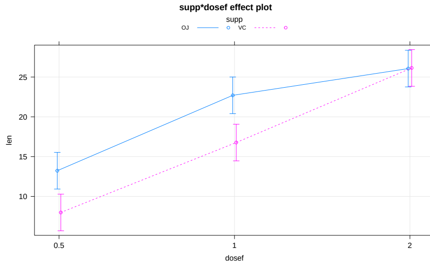
Figure 4.13: Term-plot for the estimated interaction for the Odontoblast Growth data using the multiline = T and ci.style = "bars" options.
