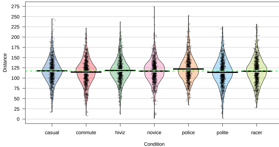
Figure 3.1: Pirate-plot of the overtake distances for the seven groups with group mean (bold lines with boxes indicating 95% confidence intervals) and the overall sample mean (dashed line) of 117.1 cm added.
