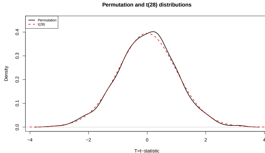
Figure 2.14: Plot of permutation and t -distribution with df = 28 . Note the close match in the two distributions, especially in the tails of the distributions where we are obtaining the p-values.
