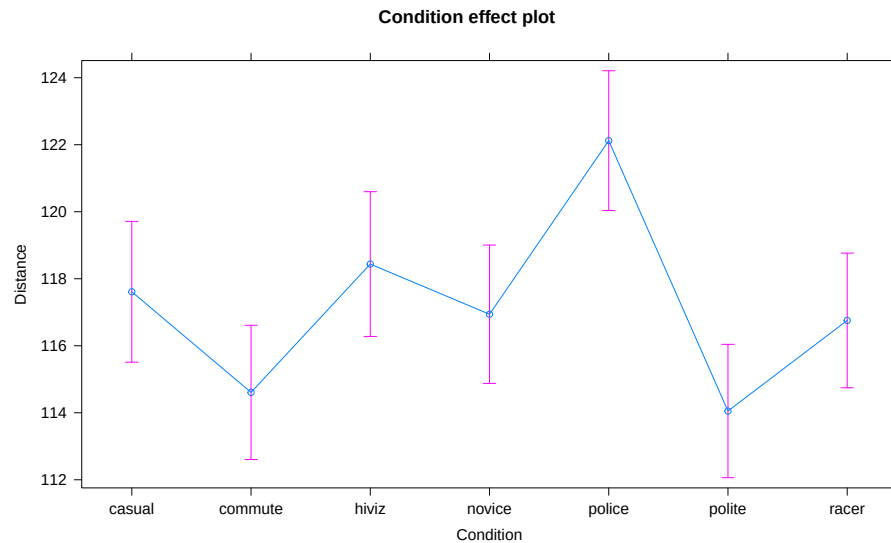
Figure 3.2: Plot of the estimated group mean distances from the reference-coded model for the overtake data from the effects package.
