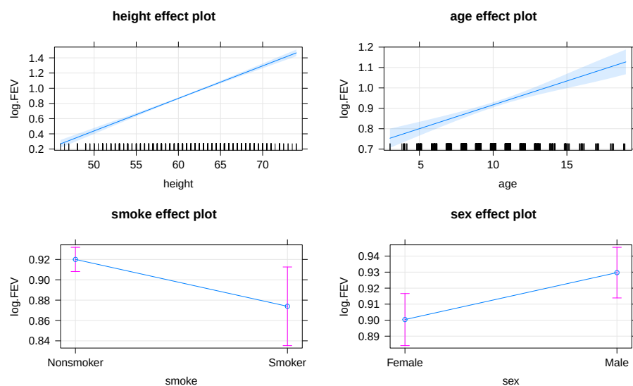
Figure 8.46: Term-plots for the top AIC model for \log(\text{FEV}) that includes height, age, smoking status, and sex in the model.
