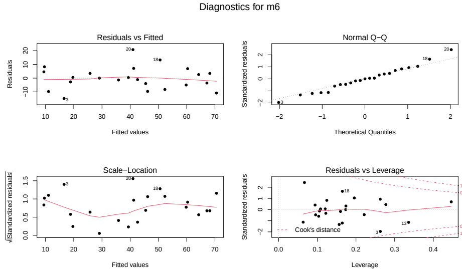
Figure 8.9: Diagnostic plots for MLR for Snow Depth based on Elevation, Min Temp and Max Temp with two observations removed ( n = 23 ).
