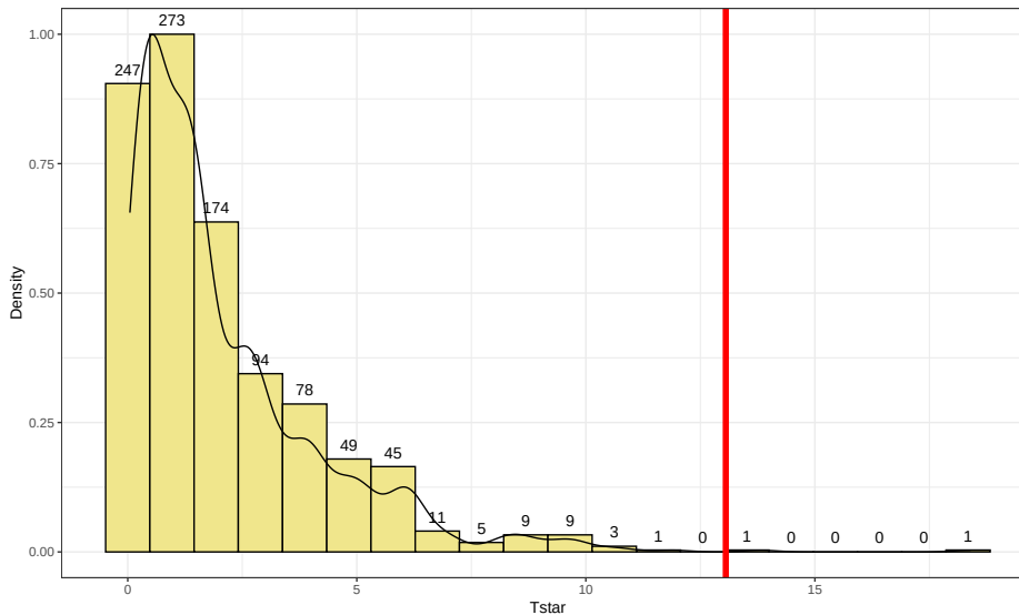
Figure 5.9: Permutation distribution for the X^2 statistic for the Arthritis data with an observed X^2 of 13.1 (bold, vertical line).
