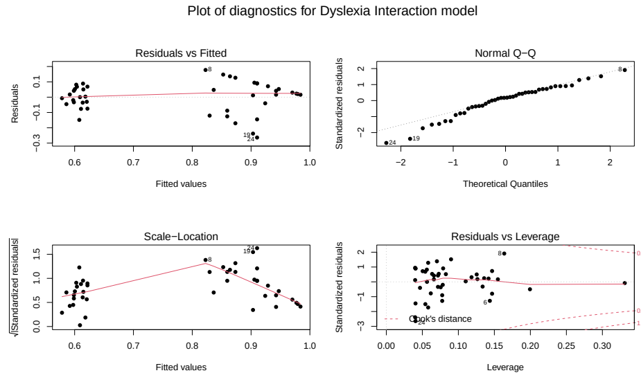
Figure 8.32: Diagnostic plots for interaction model for reading scores.
