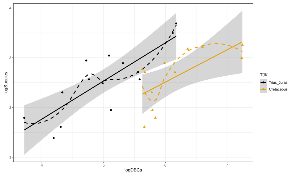
Figure 9.10: Scatterplot of log-biodiversity vs log-DBC s by TJK .
