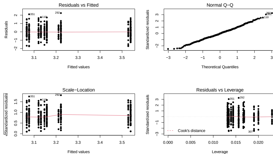
Figure 4.17: Diagnostic plot of additive model for “prodebt” by income group and whether they buy cigarettes/not.
