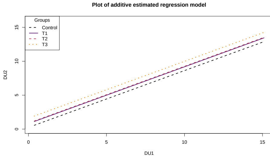
Figure 8.27: Plot of estimated noise tolerance additive model.
