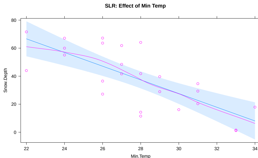
Figure 8.3: Plot of the estimated SLR model using Min Temp as predictor.
