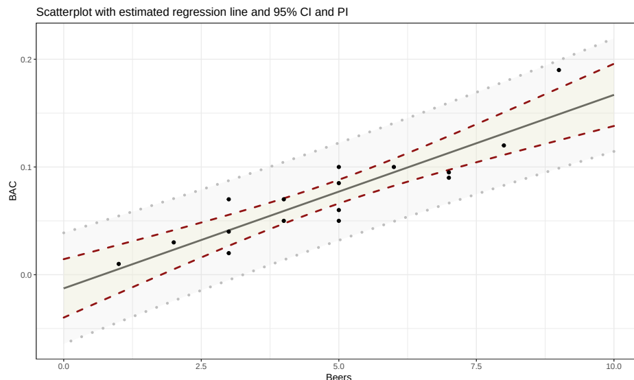
Figure 7.23: Estimated SLR for BAC data with fitted values (solid line), 95% confidence (darker, dashed lines), and 95% prediction (lighter, dotted lines) intervals.
