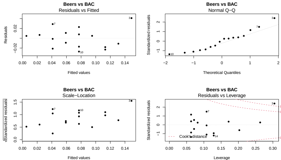
Figure 6.22: Full suite of diagnostics plots for Beer vs BAC data.
