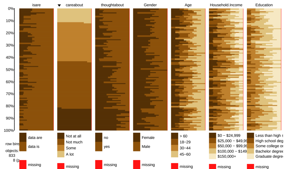
Figure 5.27: Tableplot of data from “data-is-vs-data-are” survey, sorted by “CareAbout” responses.
