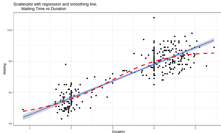
Figure 6.24: Scatterplot of Old Faithful waiting times to next eruption (minutes) and duration of prior eruption (minutes) with smoothing line (dashed) and regression line (solid).
