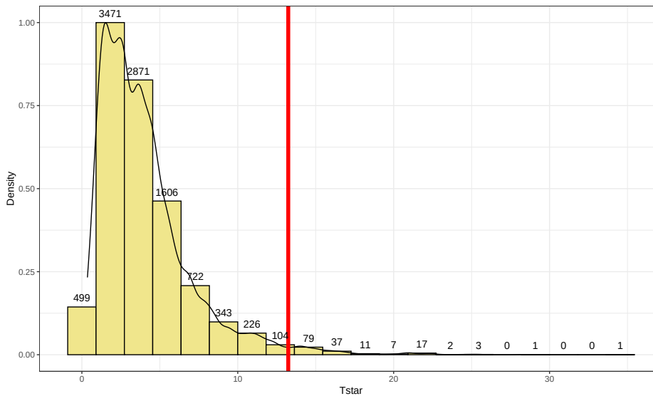
Figure 5.22: Plot of permutation distributions for cheat/lie results with observed value of 13.24 (bold, vertical line).
