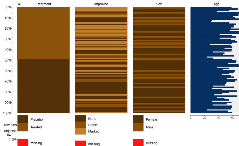
Figure 5.1: Tableplot of the arthritis data set.
