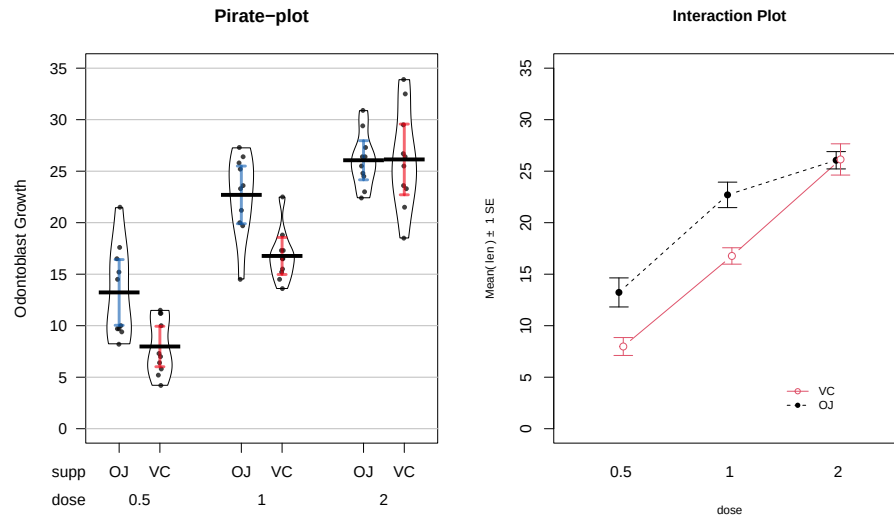
Figure 4.10: Pirate-plot and interaction plot of the odontoblast growth data set.
