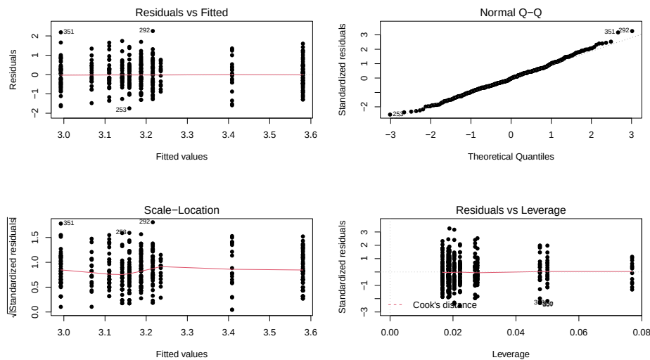
Figure 4.16: Diagnostic plot for prodebt by income group and buy cigarettes/not interaction model.
