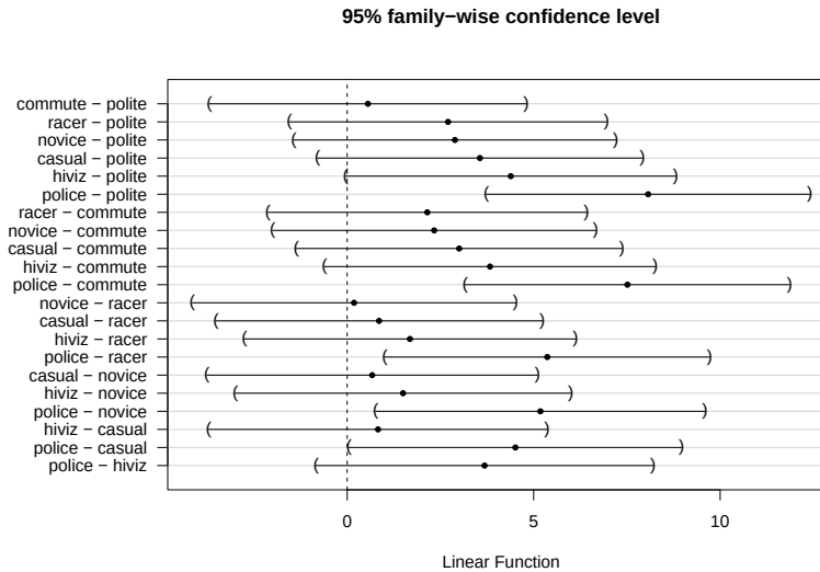
Figure 3.20: Tukey's HSD confidence interval results at the 95% family-wise confidence level for the overtake distances linear model using the new Condition2 explanatory variable.
