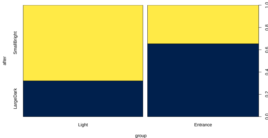
Figure 9.9: Stacked bar chart for Ant Colony results.
