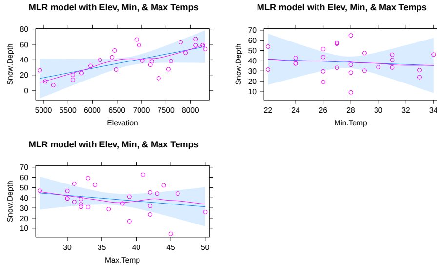
Figure 8.5: Term-plots for the MLR for Snow Depth based on Elevation, Min Temp and Max Temp. Compare this plot that comes from one MLR model to Figures 8.2, 8.3, and 8.4 for comparable SLR models. Note the points in these panels are the partial residuals that are generated after controlling for the other two of the three variables as explained below.
