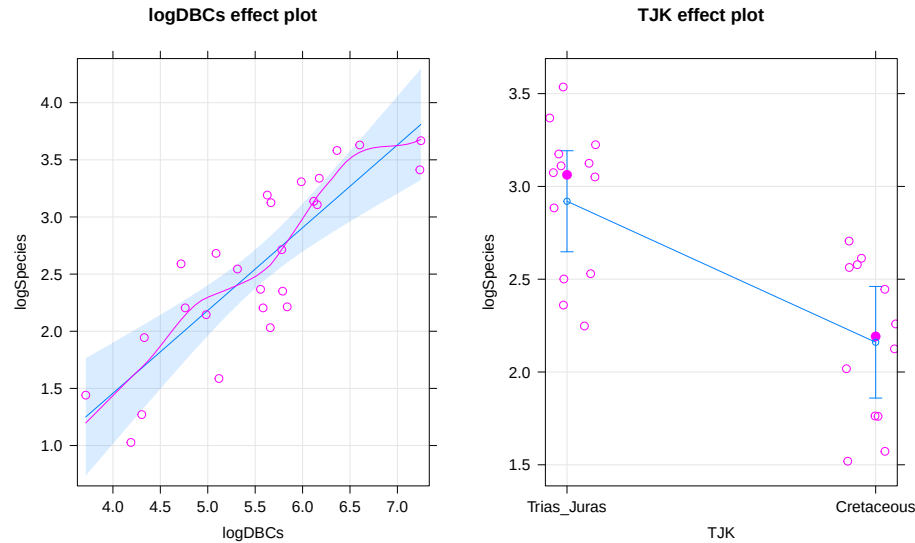
Figure 9.12: Term-plots for the top AIC model with partial residuals.
