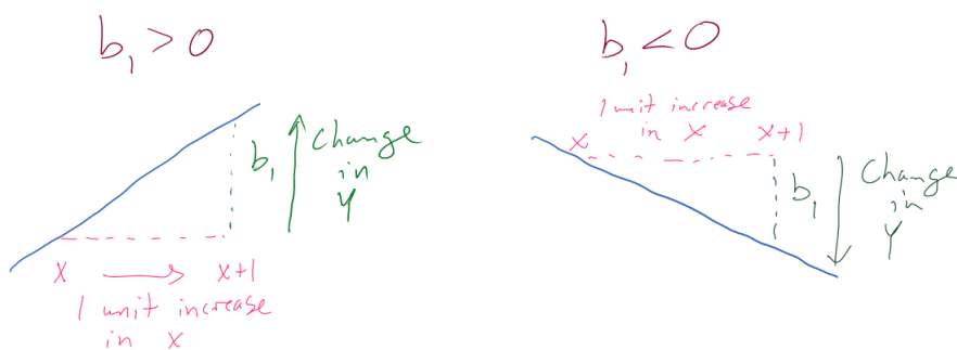
Figure 6.14: Diagram of interpretation of slope coefficients.
