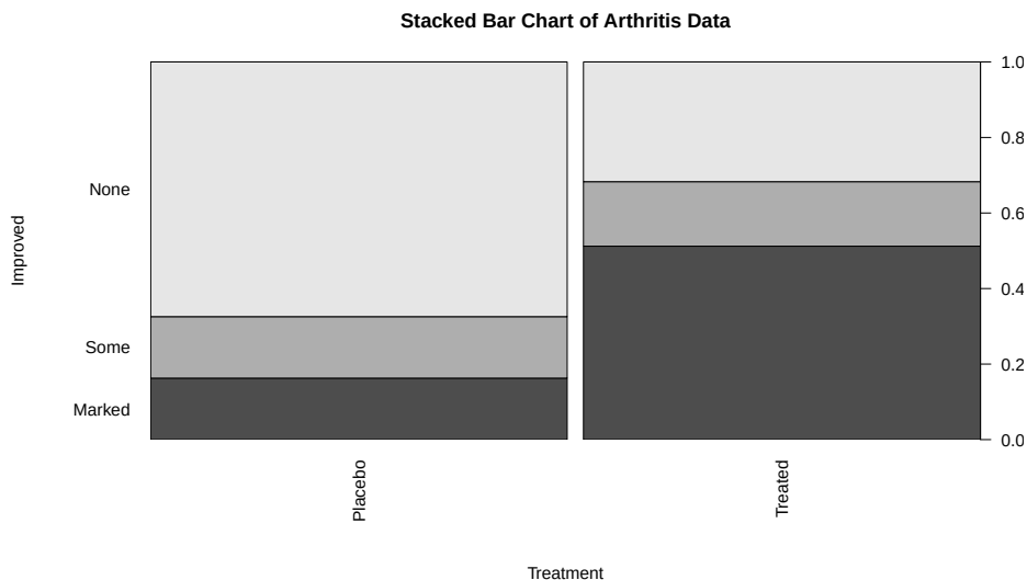
Figure 5.11: Stacked bar chart of the Arthritis data comparing Treated and Placebo .
