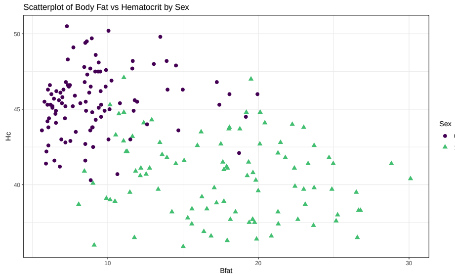
Figure 6.8: Scatterplot of athlete’s body fat and hematocrit by sex of athletes. Males were coded as 0s and females as 1s.
