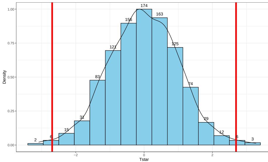
Figure 2.17: Histogram and density curve of permutation distribution of test statistic for Intermediate Statistics student GPAs.
