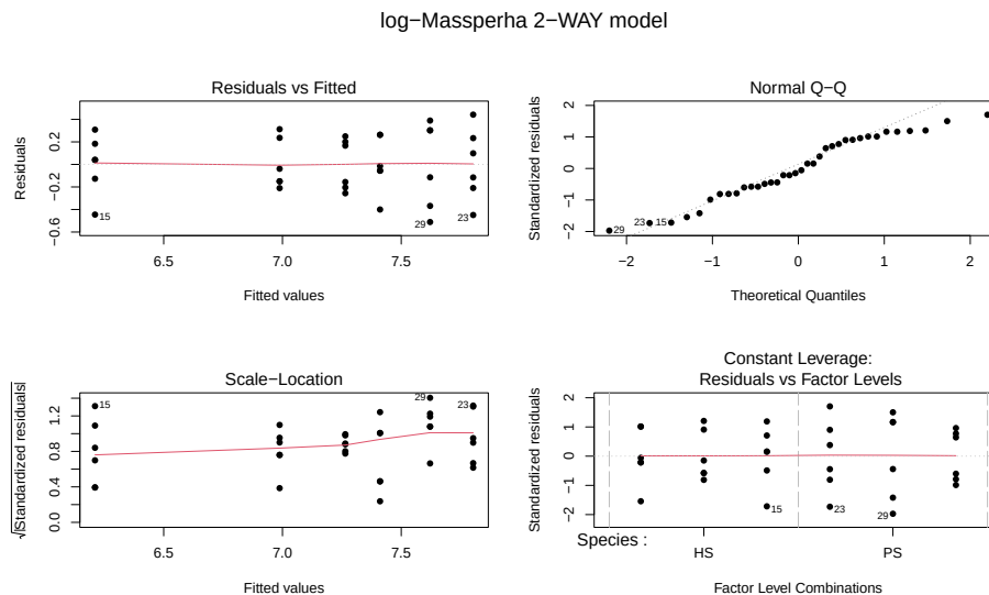
Figure 9.6: Diagnostic plots of treatment by species interaction model for log-Biomass.
