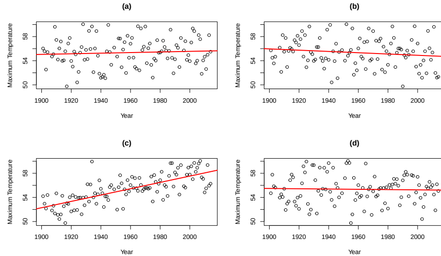
Figure 7.8: Plot of the Temperature responses versus four versions of Year , three of which are permutations of the Year variable relative to the Temperatures .
