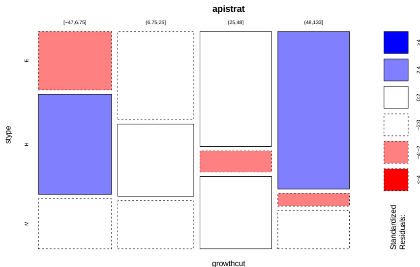
Figure 5.26: Mosaic plot of the API Growth rate categories versus level of the school with shading for size of standardized residuals.
