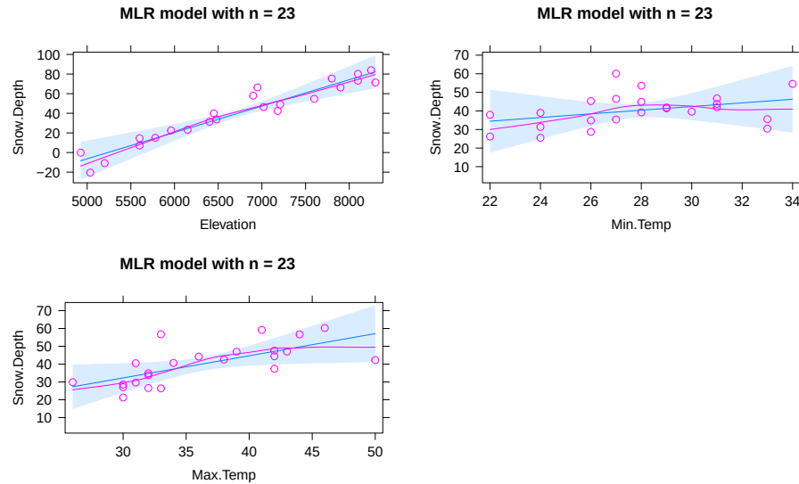
Figure 8.10: Term-plots for the MLR for Snow Depth based on Elevation, Min Temp and Max Temp with two observations removed.
