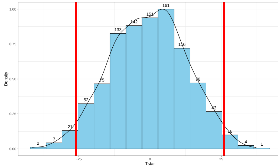
Figure 2.10: Histogram and density curve of values of test statistic for 1,000 permutations with bold lines for value of observed test statistic (-25.933) and its opposite value (25.933) required for performing the two-sided test.
