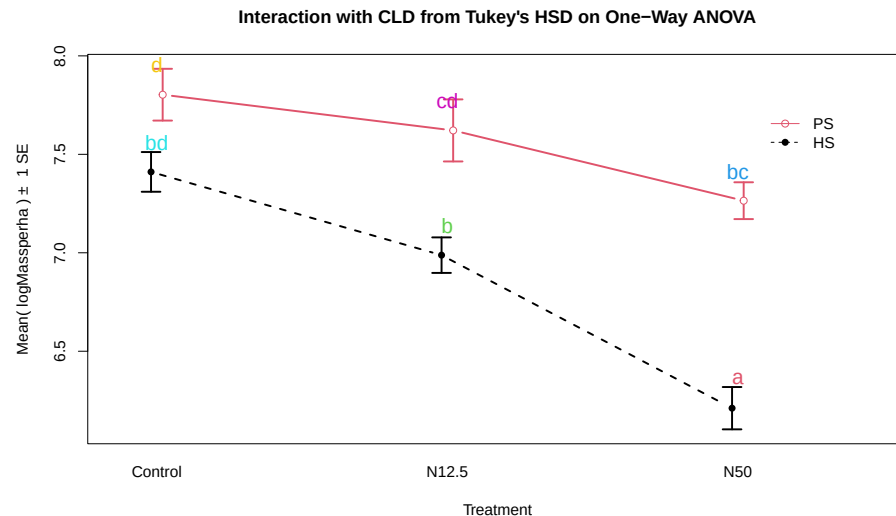
Figure 9.8: Interaction plot for log-biomass with CLD from Tukey's HSD for all pairwise comparisons.
