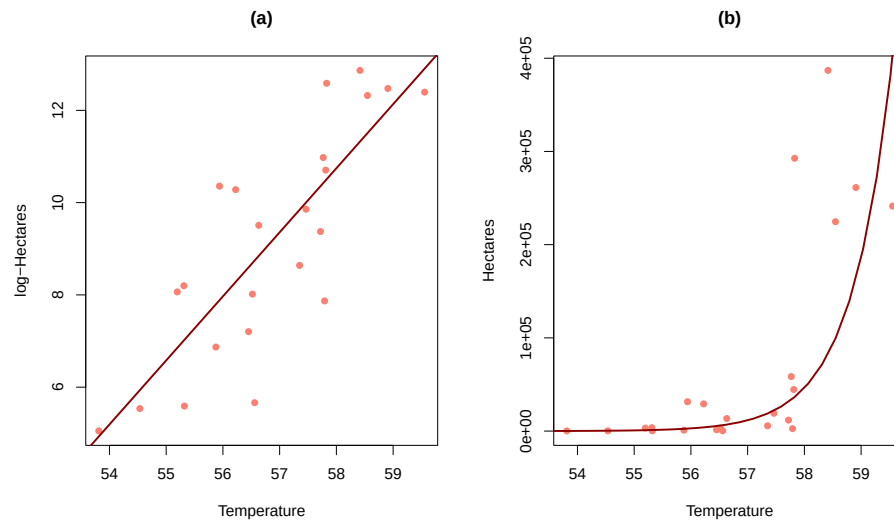
Figure 7.18: Plot of the estimated SLR (a) and implied model for the median on the original Hectares scale (b) for the area burned vs temperature data.
