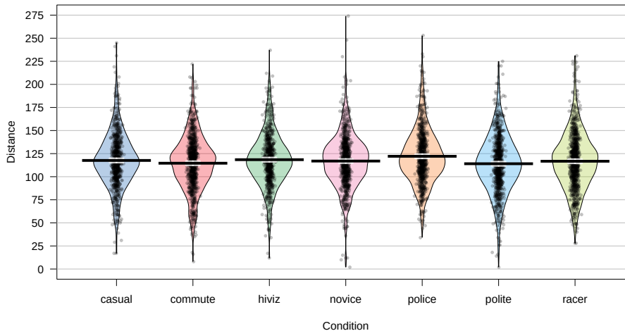
Figure 2.4: Pirate-plot of distances by outfit group. Bold horizontal lines correspond to sample mean of each group, boxes around lines (here they are very tight to the lines for the means) are the 95% confidence intervals.
