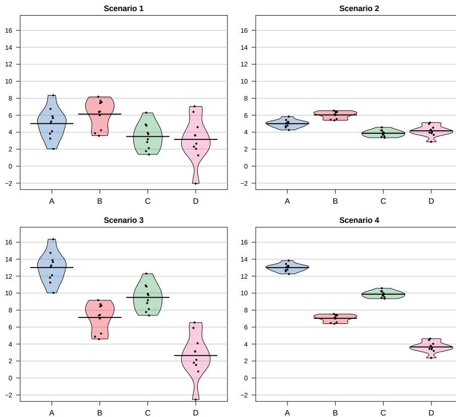
Figure 3.3: Demonstration of different amounts of difference in means relative to variability. Scenarios have the same means in rows and same variance around means in columns of plot. Confidence intervals not reported in the pirate-plots.
