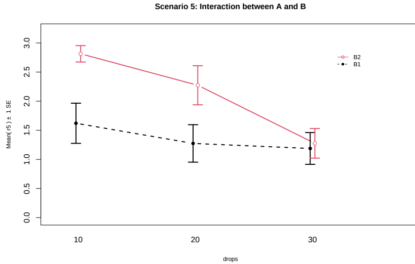
Figure 4.6: Interaction plot of Scenario 5 where it appears that an interaction is present.
