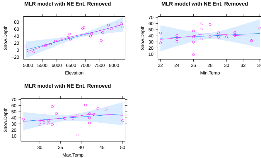
Figure 8.7: Term-plots for the MLR for Snow Depth based on Elevation, Min Temp, and Max Temp with Northeast entrance observation removed from data set ( n = 24 ).
