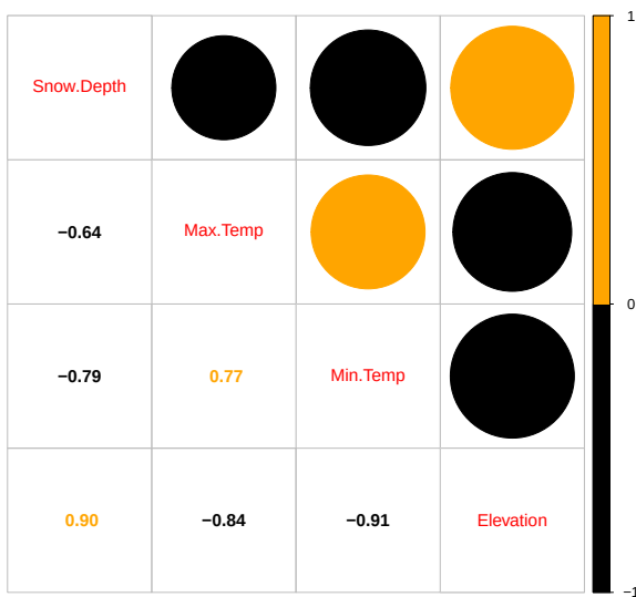
Figure 8.17: Plot of correlation matrix in the snow depth data set with influential points removed
