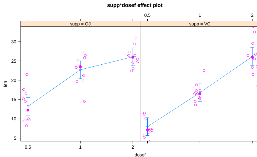
Figure 4.12: Term-plot for odontoblast growth interaction model with partial residuals added.
