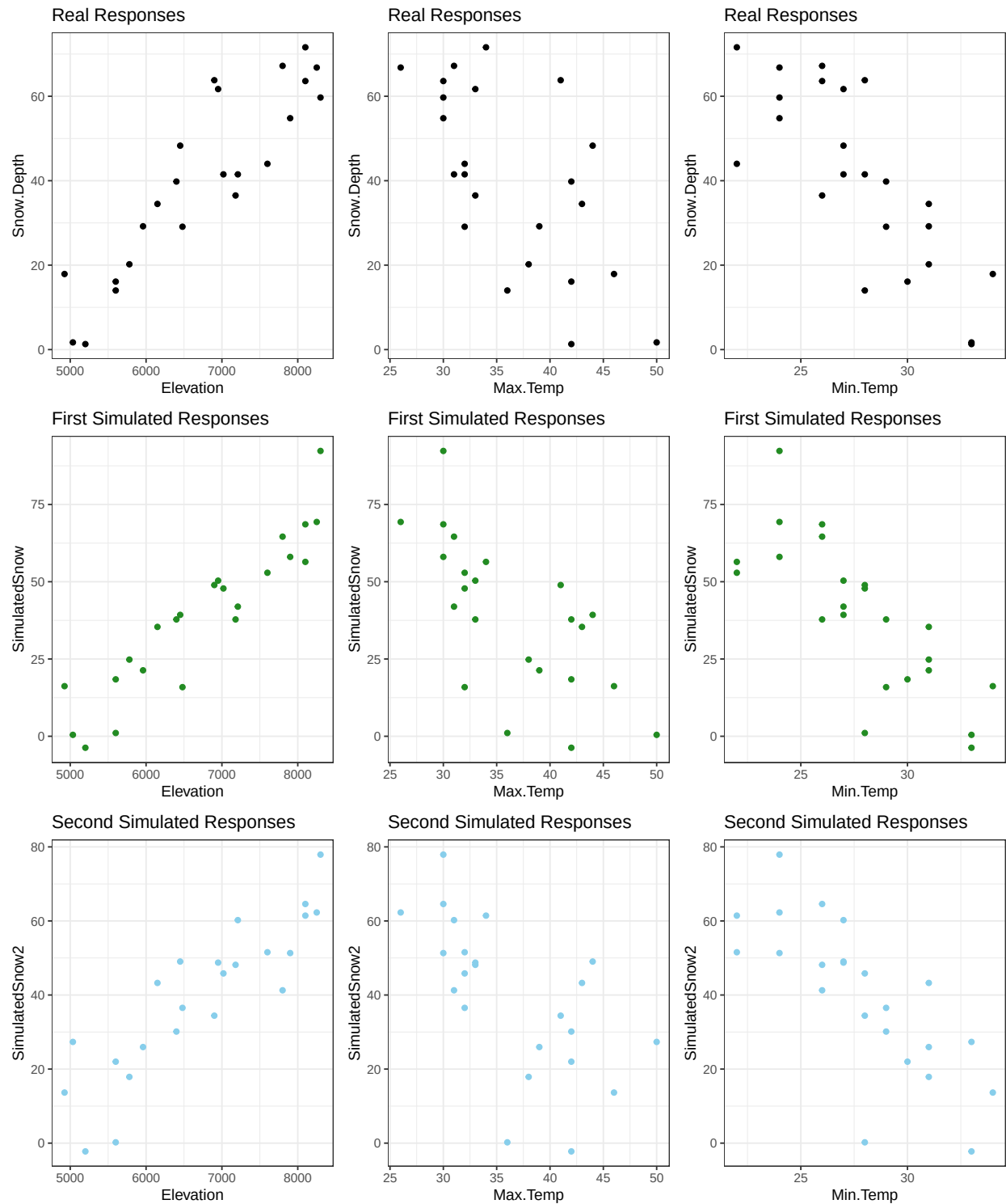
Figure 8.11: Plot of the original responses versus the three predictors ( n = 23 data set) in the top row and two sets of simulated responses versus the predictors in the bottom two rows.
