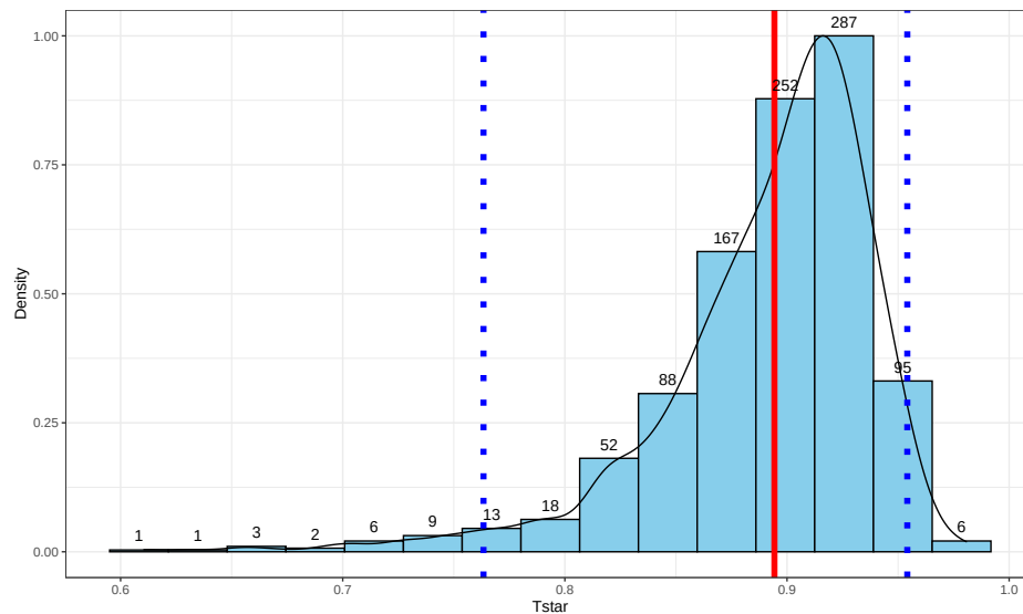
Figure 6.10: Histogram and density curve of the bootstrap distribution of the correlation coefficient with bold vertical line for observed correlation and dashed lines for bounds for the 95% bootstrap confidence interval.
