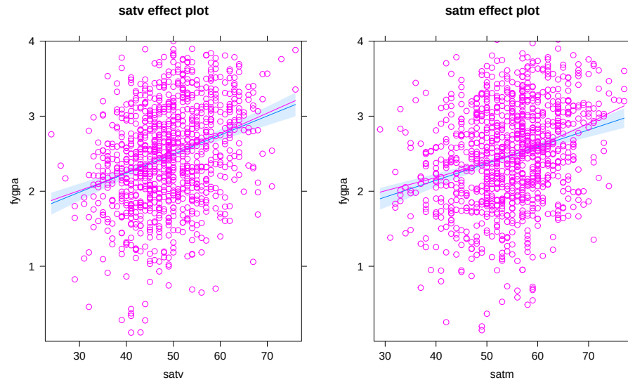
Figure 8.20: Term-plots for the fygpa \sim satv + satm model with partial residuals.
