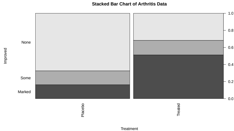
Figure 5.2: Stacked bar chart of Arthritis data. The left bar is for the Placebo group and the right bar is for the Treated group. The width of the bars is based on relative size of each group and the portion of the total height of each shaded area is the proportion of that group in each category. The lightest shading is for “none”, medium shading for “some”, and the darkest shading for “marked”, as labeled on the y-axis.
