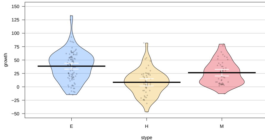
Figure 5.23: Pirate-plot of the API growth scores by level of school in the stype variable (coded E for elementary, M for Middle, and H for High school).
