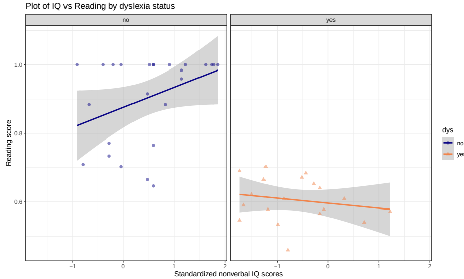
Figure 8.31: Scatterplot for reading score versus nonverbal IQ by dyslexia group.
