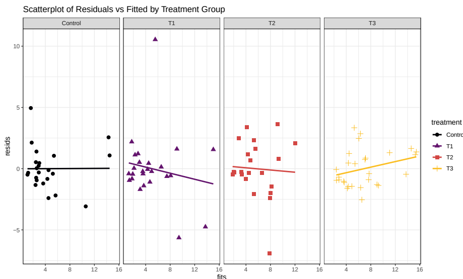
Figure 8.30: Faceted scatterplot of residuals versus fitted values by treatment group from the additive decibel tolerance model.
