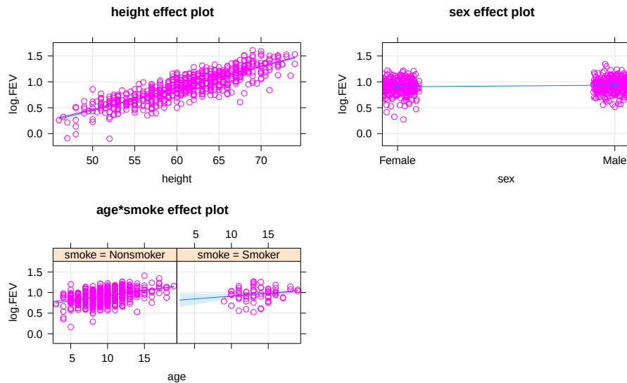
Figure 8.44: Term-plots for the \log(\text{FEV}) model that includes height, sex, and an interaction between age and smoking status (the full model), with partial residuals.
