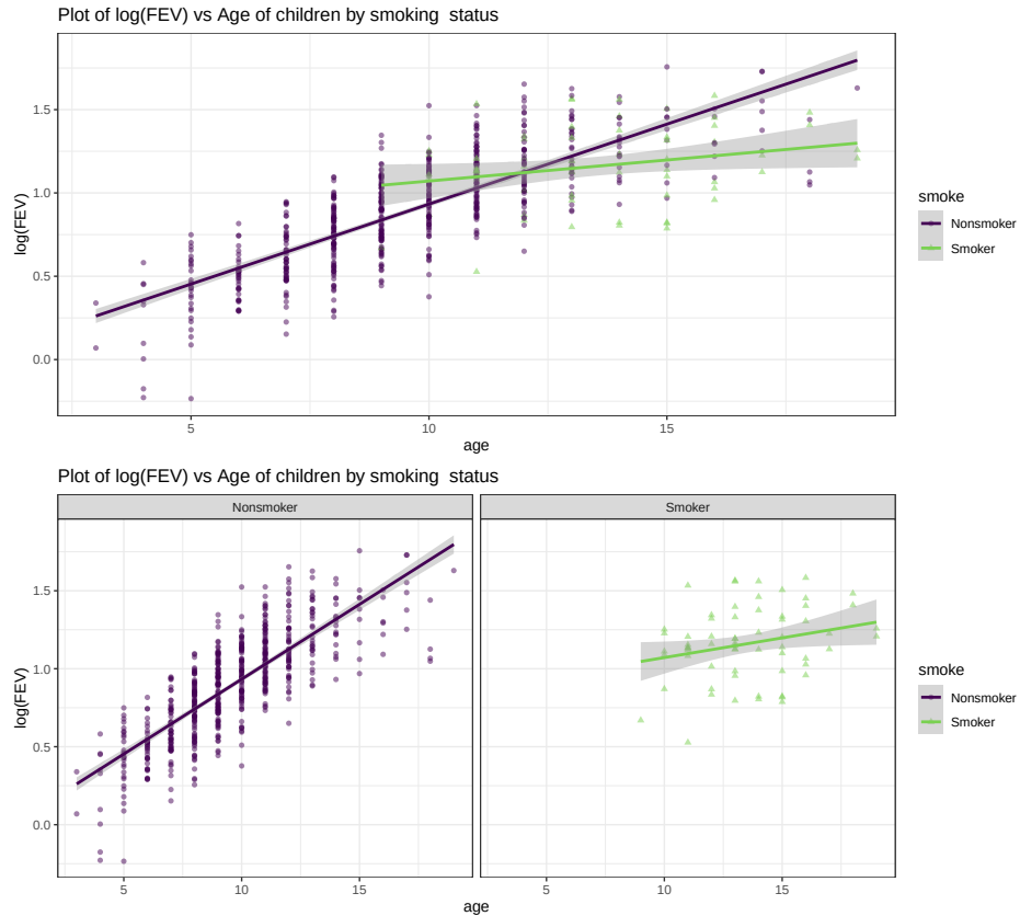
Figure 8.42: Scatterplot of log(FEV) vs Age by smoking status, with both combined (top) and faceted (bottom) versions.
