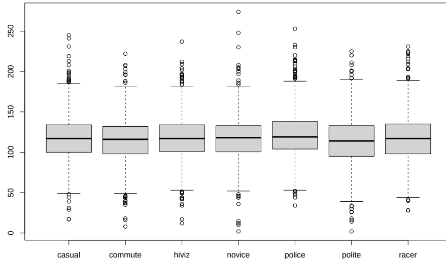
Figure 2.3: Side-by-side boxplot of distances based on outfits.
