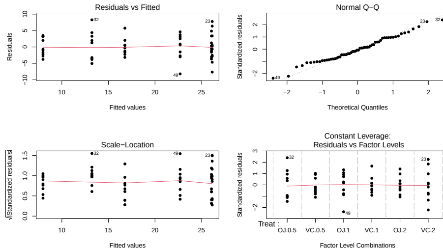
Figure 3.15: Diagnostic plots for the odontoblast growth model.
