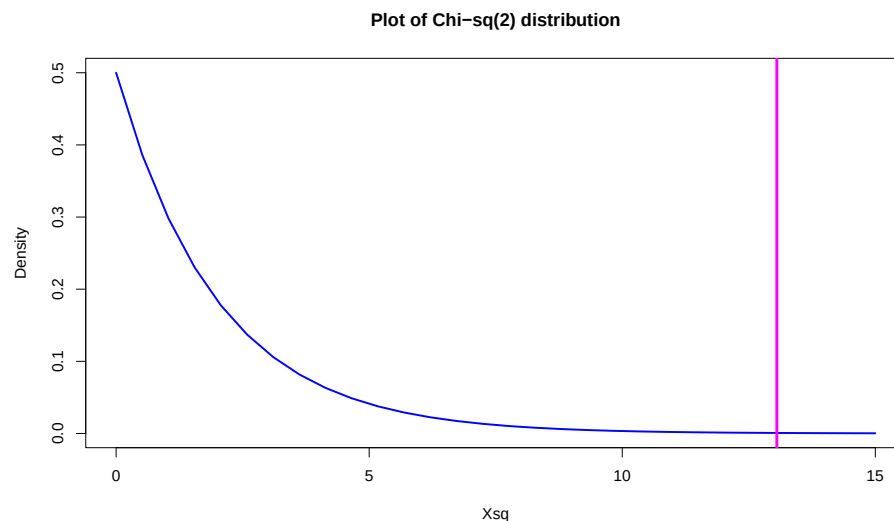
Figure 5.10: \chi^2 -distribution with two degrees of freedom with the observed statistic of 13.1 indicated with a vertical line.
