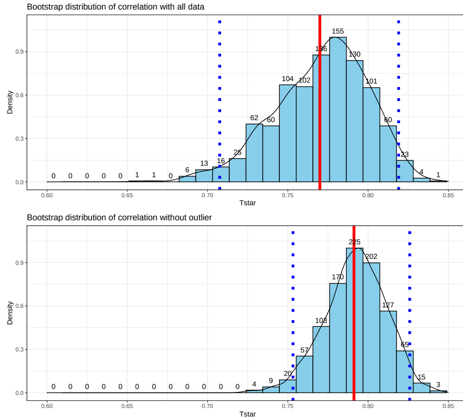
Figure 6.12: Bootstrap distributions of the correlation coefficient for the full data set (top) and without potential outlier included (bottom) with observed correlation (bold line) and bounds for the 95% confidence interval (dashed lines). Notice the change in spread of the bootstrap distributions as well as the different centers.
