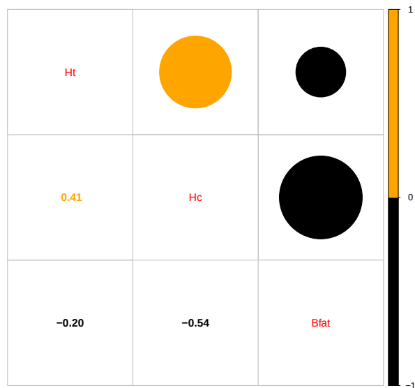
Figure 6.6: Correlation plot of the athlete data with two potential outliers removed. Lighter (orange) circle for positive correlations and black for negative correlations.
