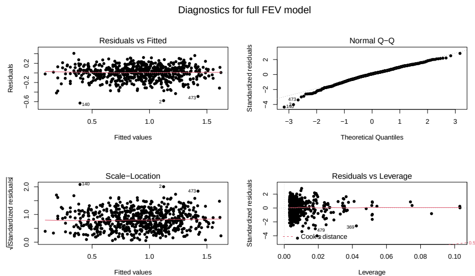
Figure 8.43: Diagnostics for the \log(\text{FEV}) model that includes height, sex, and an interaction between age and smoking status (the full model).
