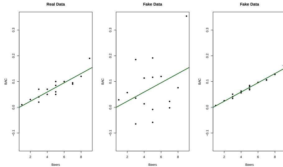
Figure 6.19: Three scatterplots with the same estimated regression line.
