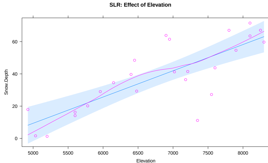
Figure 8.2: Plot of the estimated SLR model for Snow Depth with Elevation as the predictor along with observations and smoothing line generated by the residuals = T option being specified.
