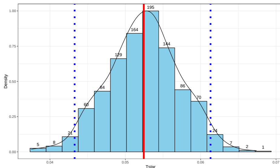
Figure 7.10: Bootstrap distribution of the slope coefficient in the Bozeman temperature linear regression model with bold dashed vertical lines delineating the 95% confidence interval and the bold solid line the observed slope of 0.052.
