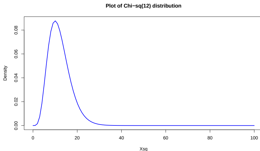
Figure 5.15: Plot of \chi^2 -distribution with 12 degrees of freedom.
