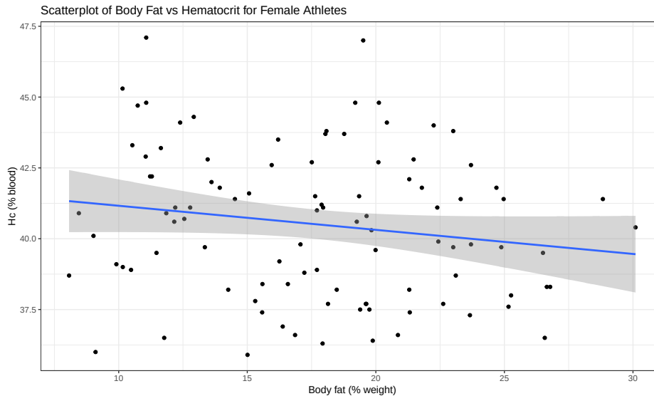
Figure 6.15: Scatterplot of Hematocrit versus Body Fat for female athletes. Note how the filter was used to pipe the subset of the data set to the plot.
