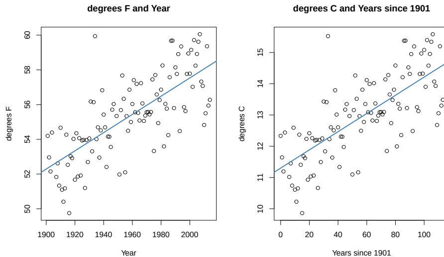
Figure 7.11: Scatterplots of Temperature ( ^{\circ}F ) versus Year (left) and Temperature ( ^{\circ}C ) vs Years since 1901 (right).
