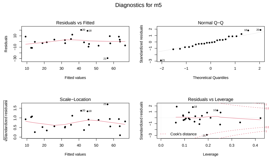
Figure 8.8: Diagnostic plots for MLR for Snow Depth based on Elevation, Min Temp and Max Temp with Northeast entrance observation removed from data set.
