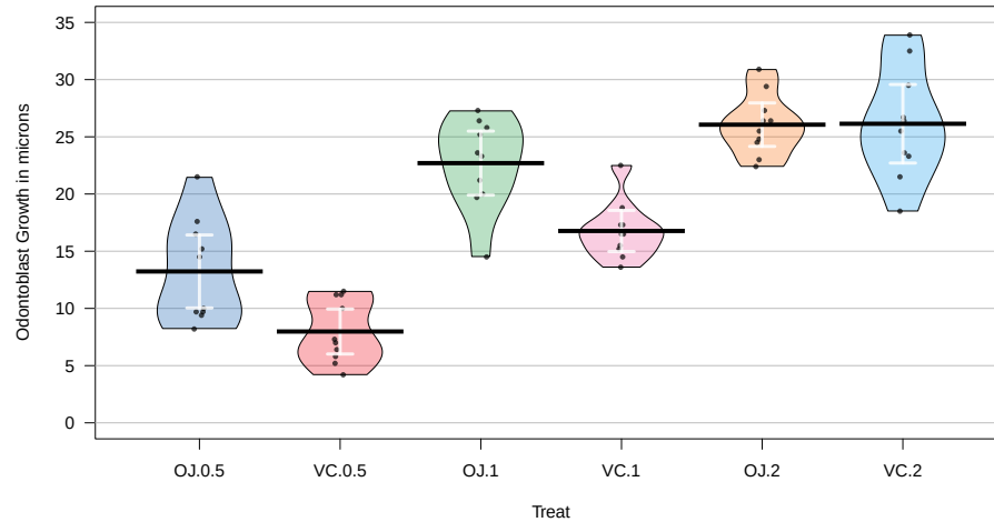
Figure 3.14: Pirate-plot of odontoblast growth responses for the six treatment level combinations.
