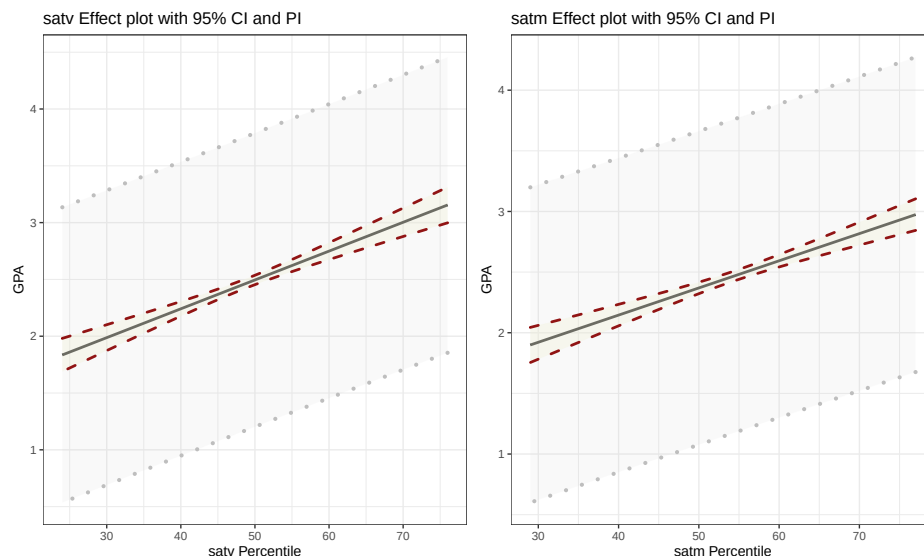
Figure 8.21: Term-plots for the \text{fygpa} \sim \text{satv} + \text{satm} model with 95% confidence intervals (dark, dashed lines) and 95% PIs (light grey, dotted lines).
