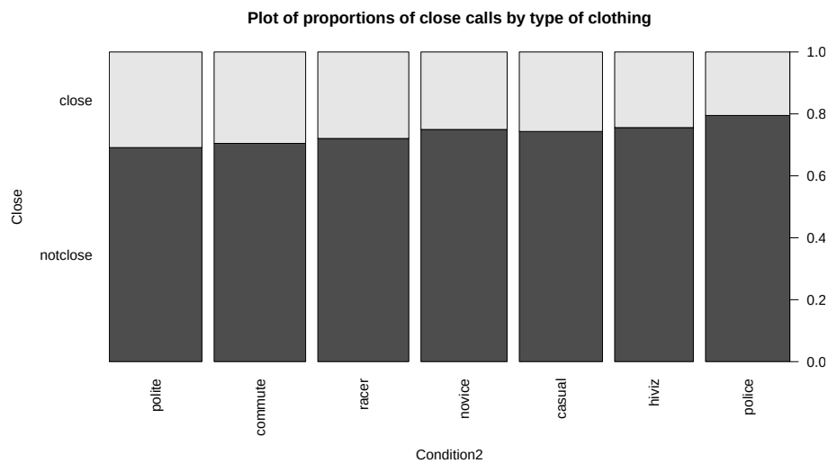
Figure 5.28: Stacked bar chart of the close calls/not (overtakes less than or equal to 100 cm or not) by outfit.
