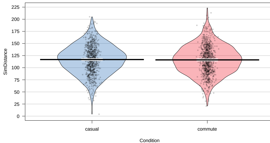
Figure 2.18: Pirate-plot of a simulated data set that assumes the same mean for both groups. The means in the two groups are very similar.
