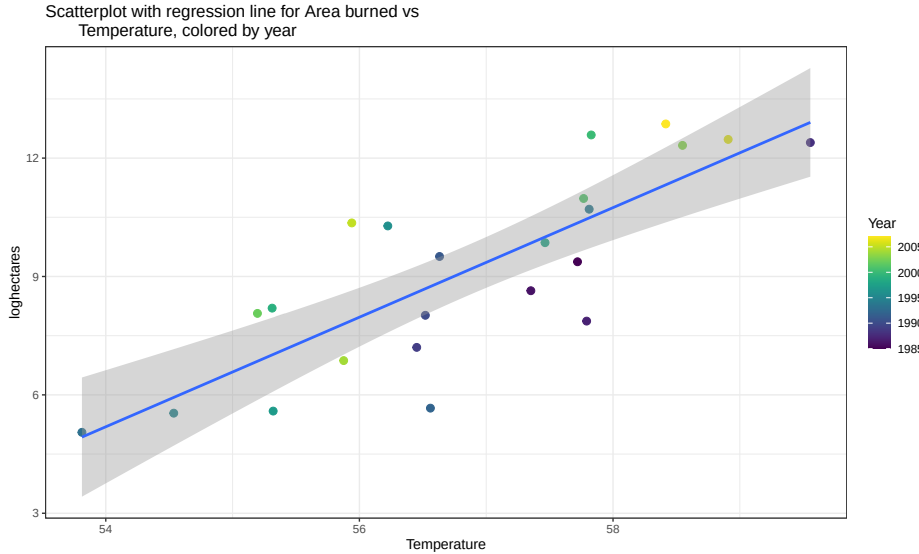
Figure 6.18: Scatterplot of log-hectares burned versus temperature with estimated regression line. Information on the year of each observation is added using a local aesthetic inside geom_point to color the points on a color gradient based on Year .
