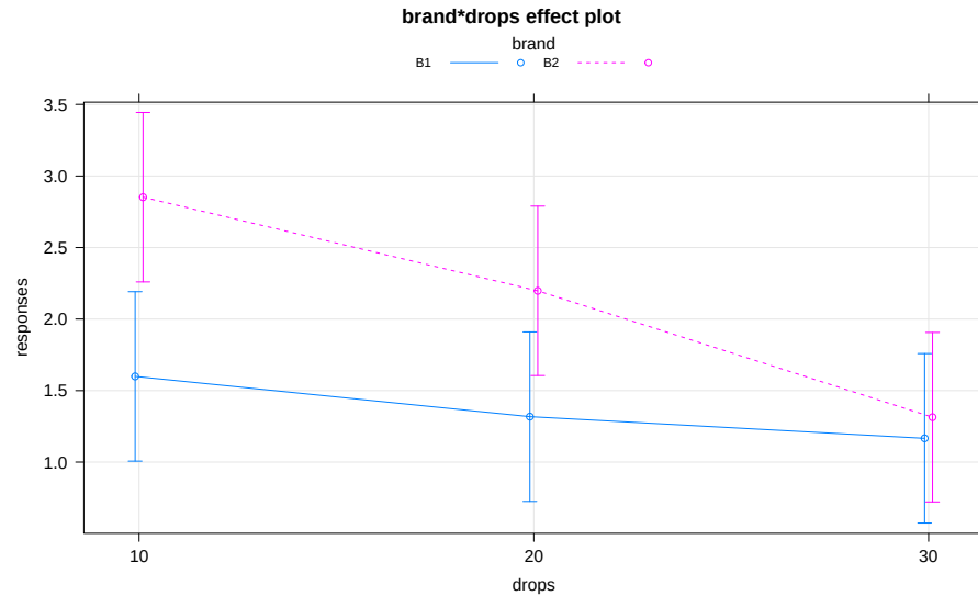
Figure 4.7: Plot of estimated results of interaction model for the paper towel performance data.
