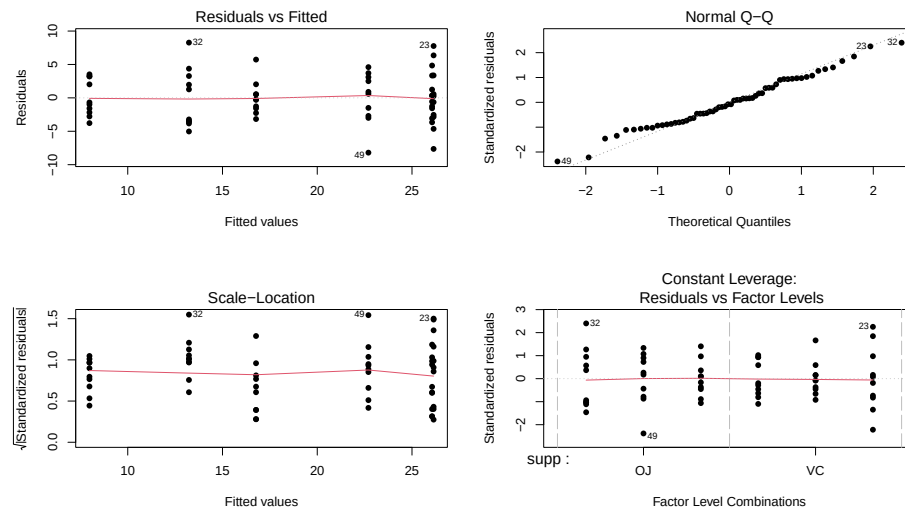
Figure 4.11: Diagnostic plots for the interaction model for odontoblast growth interaction model.
