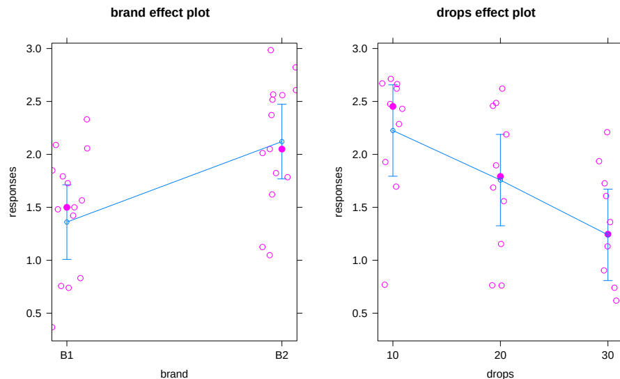
Figure 4.9: Term-plots of additive model for paper towel data with partial residuals added. Relatively similar variability seems to be present in each of the groups of residuals after adjusting for the other variable except for the residuals for the 10 drops where the variability is smaller, especially if one small outlier is ignored.
