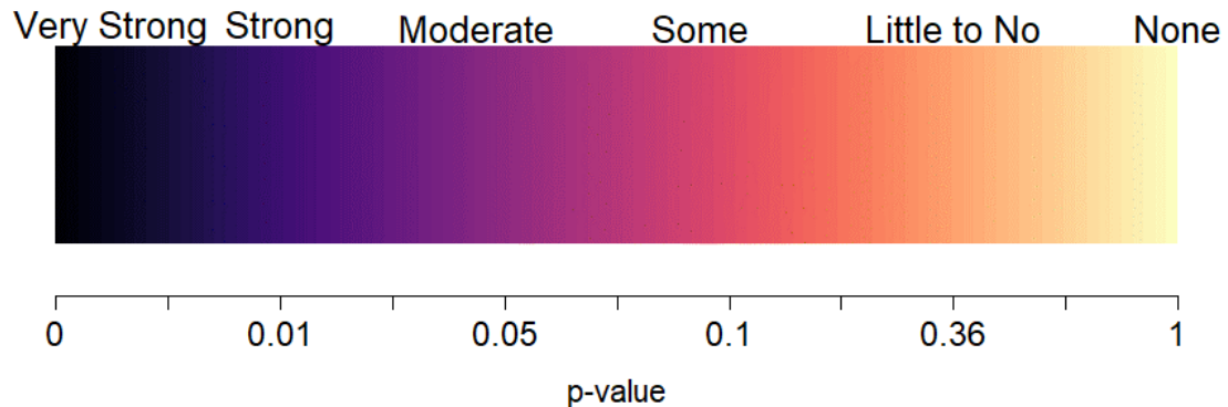
Figure 2.11: Graphic suggesting potential interpretations of strength of evidence based on gradient of p-values. P-values range from 0 to 1, with only a p-value of 1.0 providing no evidence against the null hypothesis.
