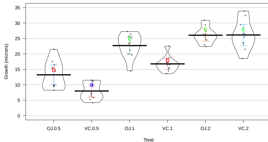
Figure 3.19: Pirate-plot of odontoblast growth by group with Tukey’s HSD compact letter display. Note some extra pirate-plot options are used to enhance focus on the CLD results.
