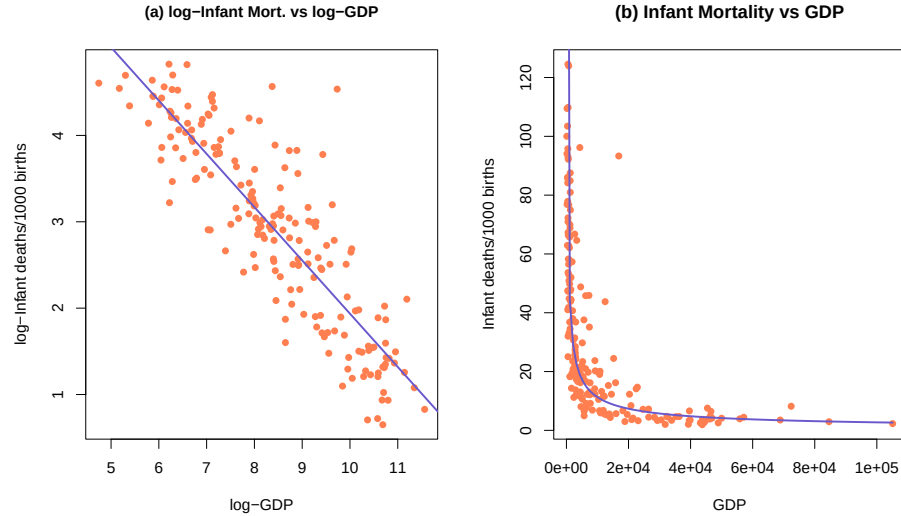
Figure 7.21: Plot of the observations and estimated SLR model \log(\text{mortality}) \sim \log(\text{GDP}) (left) and implied model (right) for the infant mortality data.
