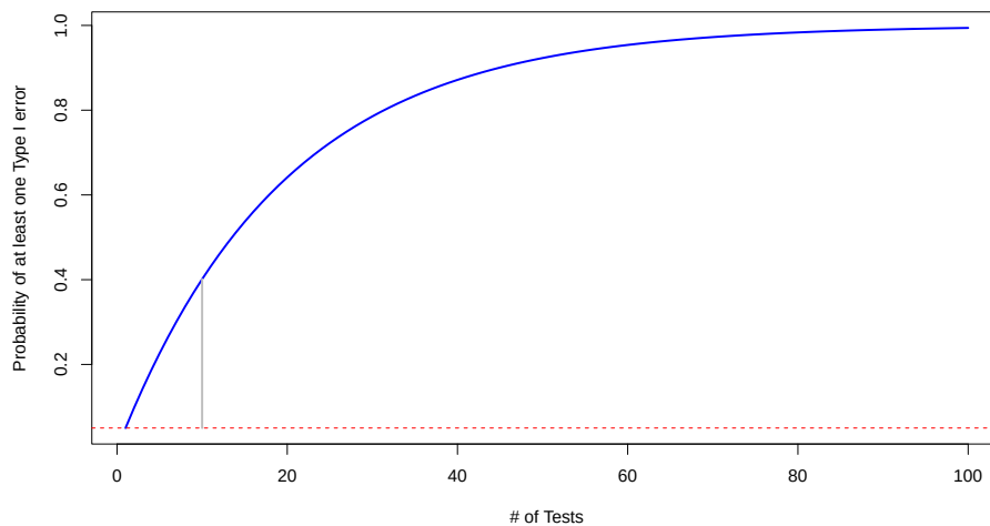
Figure 2.20: Plot of family-wise error rate (bold solid line) as the number of tests performed increases. Dashed line indicates 0.05 and grey solid line highlights the probability of at least on error on m = 10 tests.
