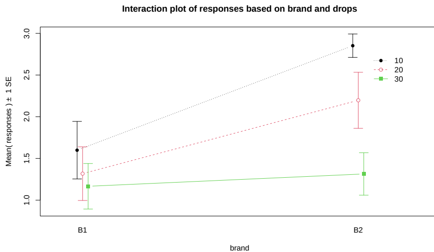
Figure 4.3: Interaction plot of paper towel data with Brand on the x-axis and lines based on Drops .
