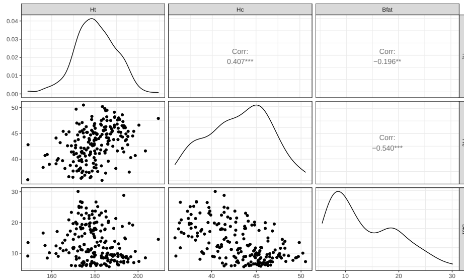
Figure 6.5: Scatterplot matrix of athlete data with two potential outliers removed.
