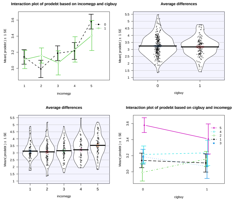
Figure 4.15: Interaction plot array of prodebt by income group (1 to 5) and whether they buy cigarettes (0 = no, 1 = yes).
