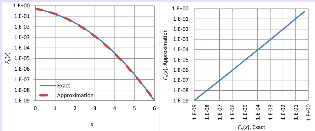
Figure 5.5 Comparison of the approximation of the normal distribution by equation (5.45) with the exact normal distribution.
