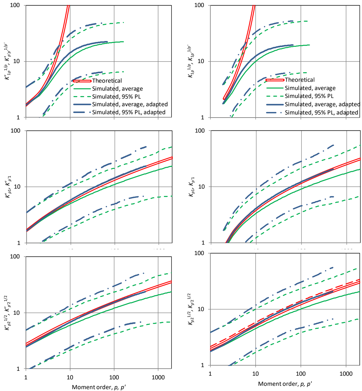
Figure 6.17 Illustration of the performance of the adaptation of K-moment estimation for an HK process with Hurst parameter 0.9 and lognormal marginal distribution (LN(0,1); same as in Figure 6.4, left): (left column) noncentral moments; (right column) central moments; (middle row) q = 1 (bottom row) q = 2 . For comparison classical moments are also shown ( upper row ). The estimates are averages of 200 simulations each with n = 2000 and are almost indistinguishable from the theoretical values. The first-order approximation of equation (6.119) was used for the adaptation. For K_{p2} ( lower right ) the true K-moments are represented by the dashed curve while the curve marked “theoretical” corresponds to the true plus bias, where bias is determined from equation (6.124). The 95% prediction limits (PL) are also shown.
